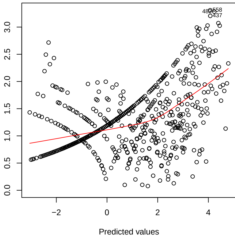
Scale-Location
