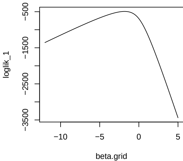
alpha = 1
