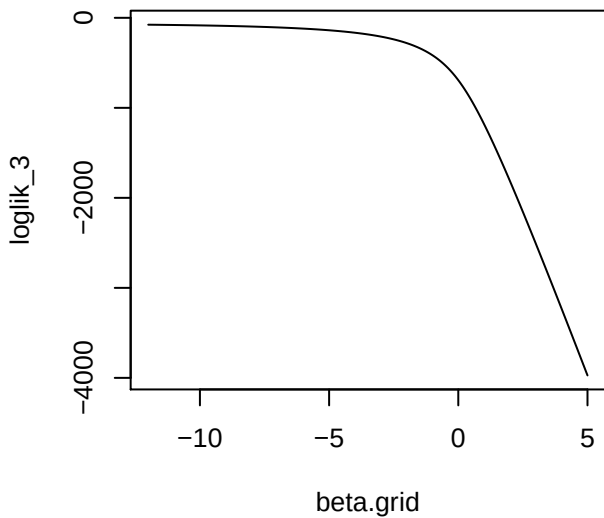
alpha = 0.1
