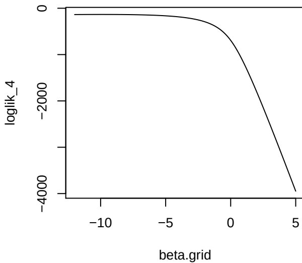
alpha = 0
