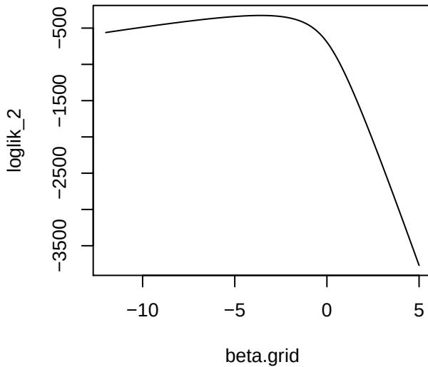
alpha = 0.5
