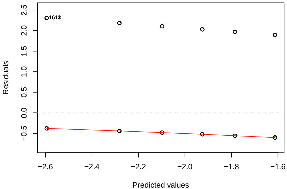
Bernoulli Residuals vs Fitted
