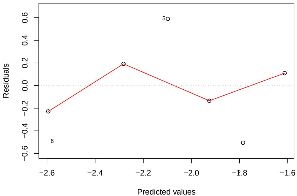
Binomial Residuals vs Fitted
