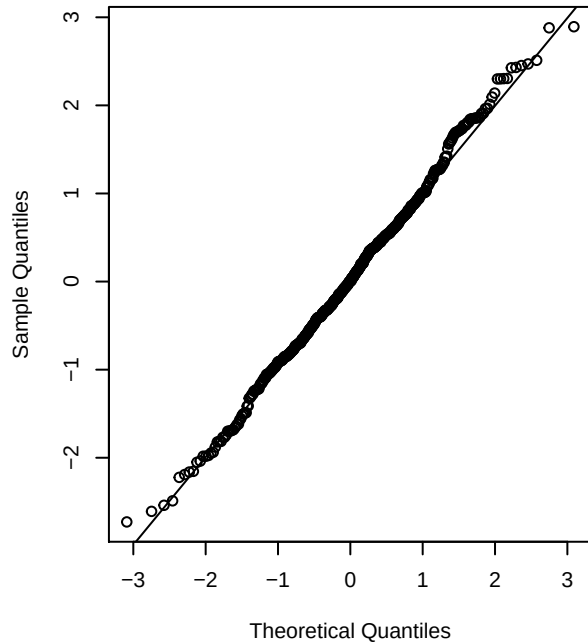
Binomial, m = 10
