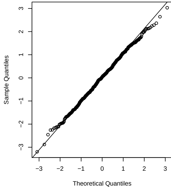
Binomial, m = 100
