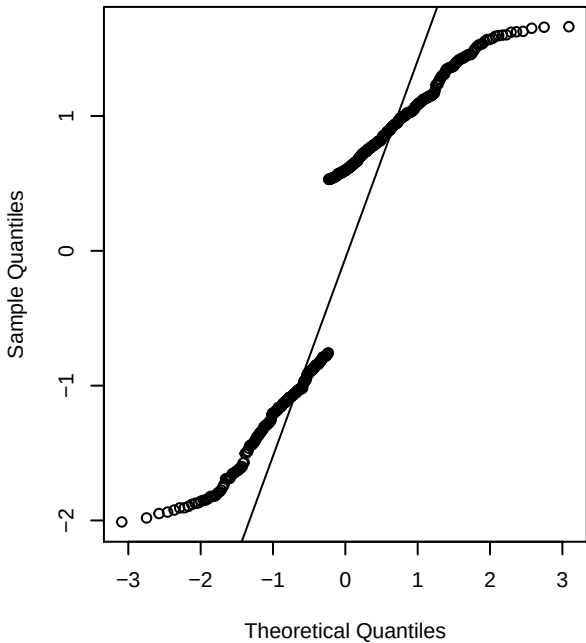
Bernoulli
