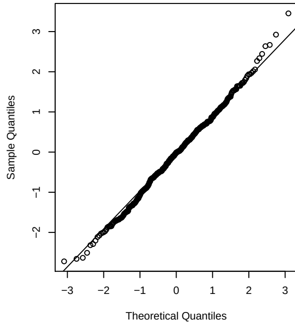
Poisson, high lambda
