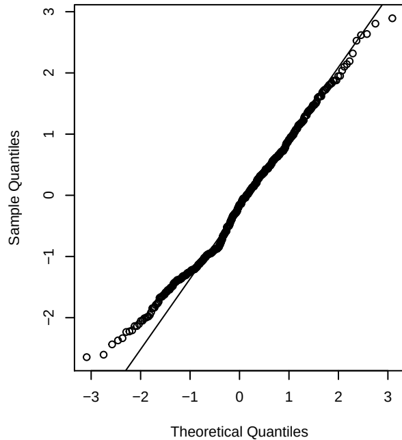
Poisson, typical case
