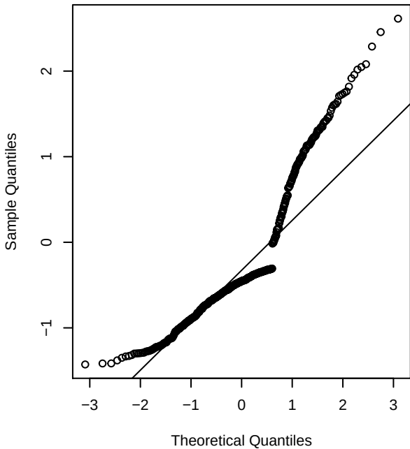
Poisson, low lambda
