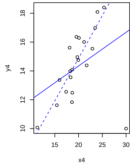
High Residual and Leverage
