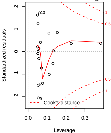
Residuals vs Leverage
