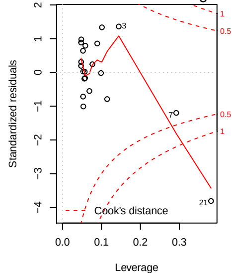
Residuals vs Leverage
