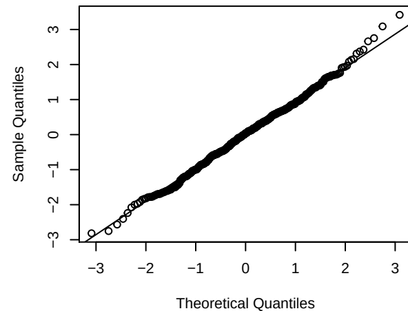
Poisson, high lambda
