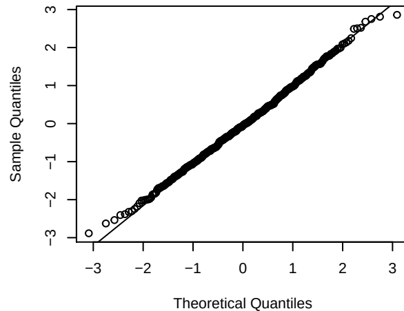
Poisson, typical case
