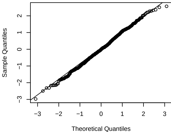
Poisson, low lambda
