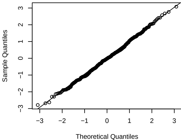
Bernoulli
