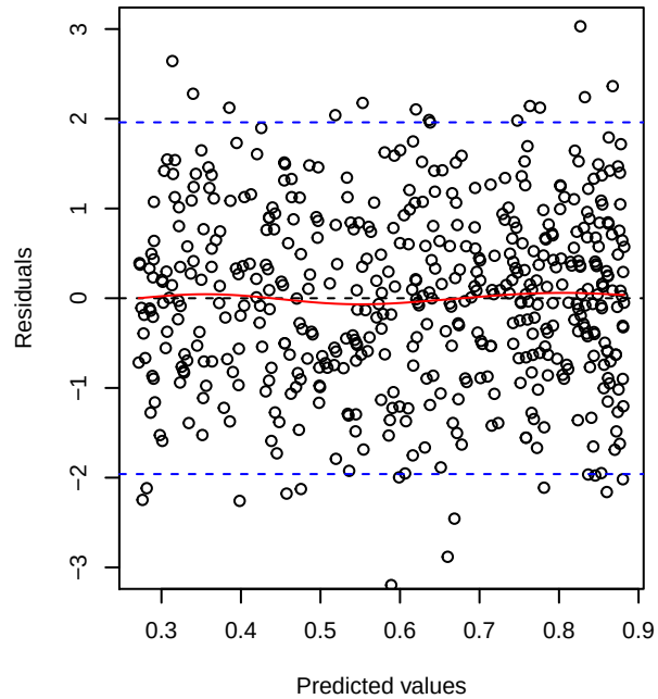
Binomial, m = 100
