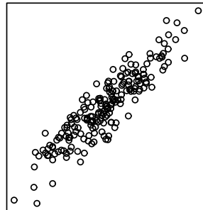
Corrélation = 0.9
