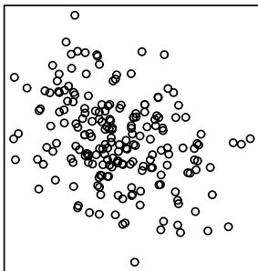
Corrélation = -0.3
