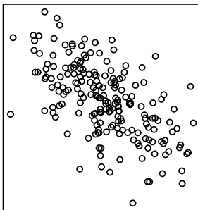
Corrélation = -0.6
