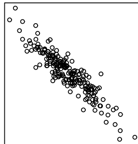
Corrélation = -0.9
