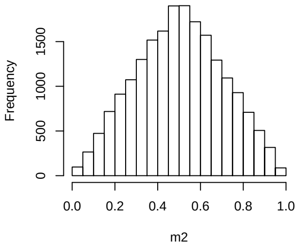
Histogram of m2
