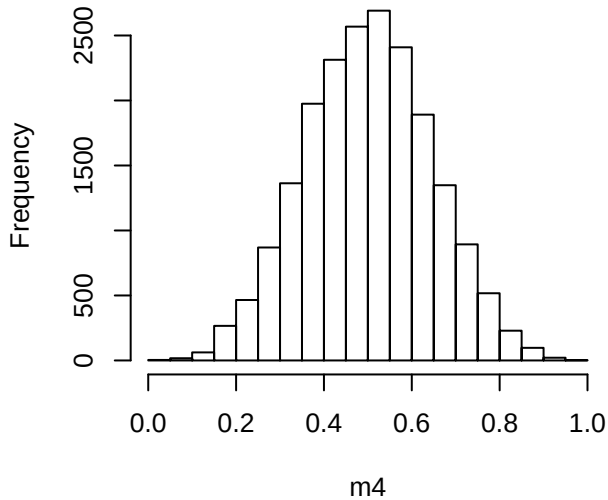
Histogram of m4
