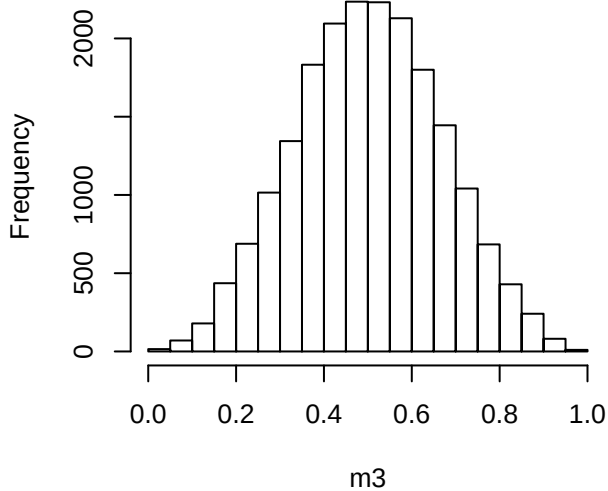
Histogram of m3
