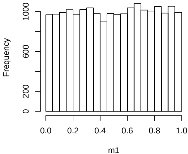
Histogram of m1
