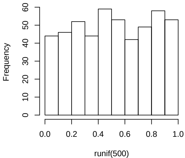
Histogram of runif(500)
