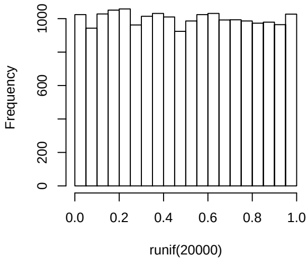
Histogram of runif(20000)
