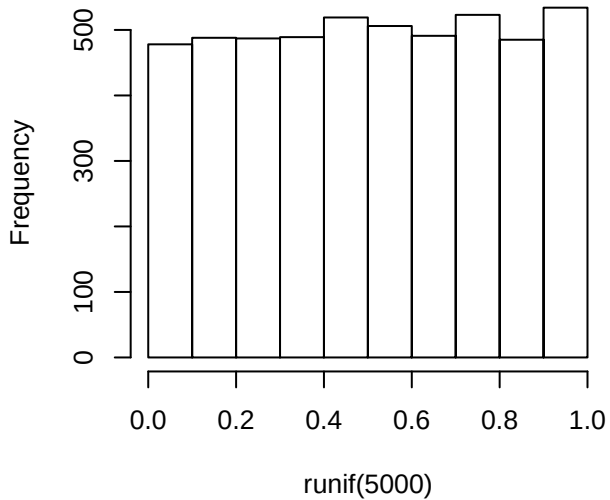
Histogram of runif(5000)
