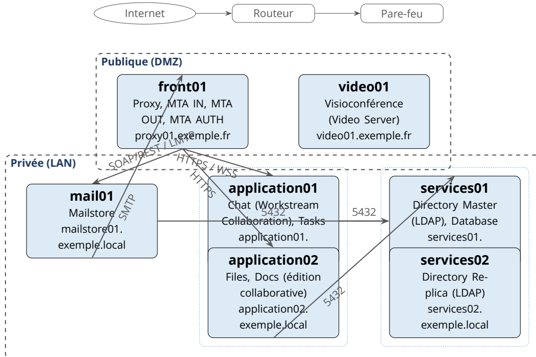
Figure 5.6 – Flux — Flux applicatif interne (SOAP / REST)
