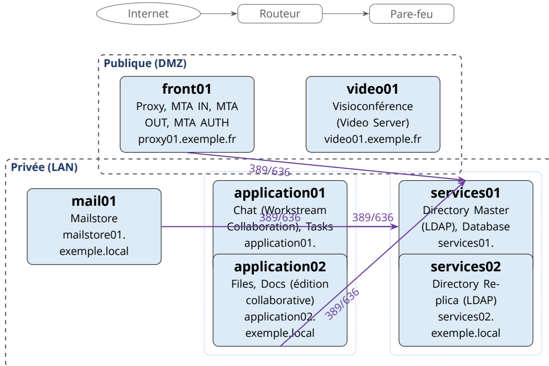
Figure 5.4 – Flux — Service Discover / LDAP
