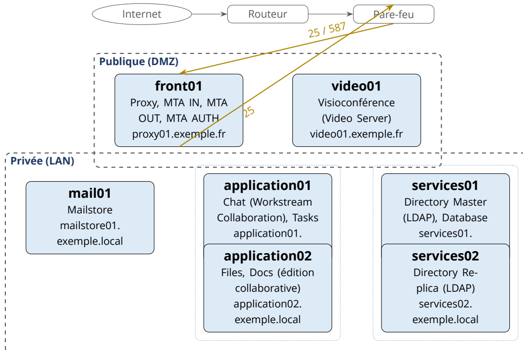
Figure 5.3 – Flux — SMTP
