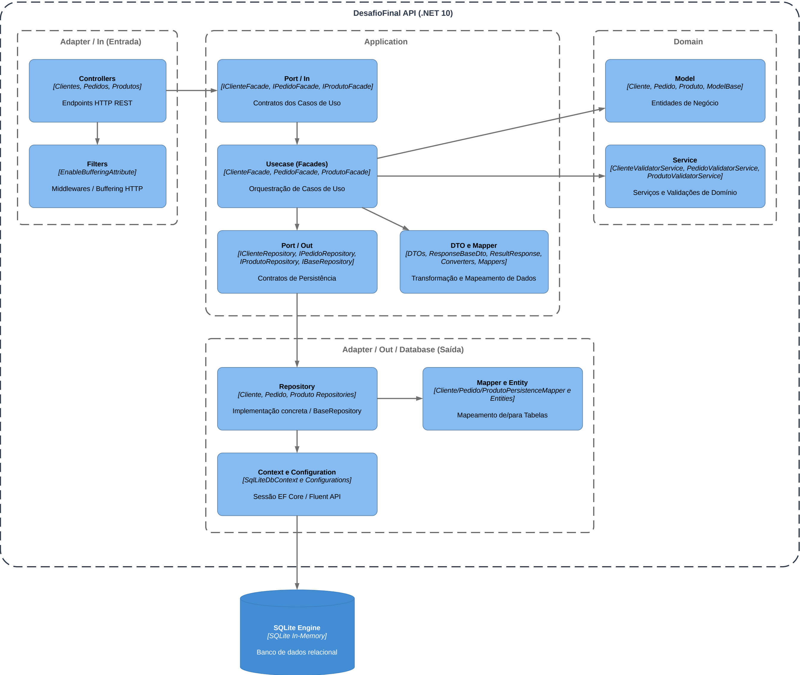
Diagrama de Componentes - DesafioFinal API (Hexagonal / Ports e Adapters)
