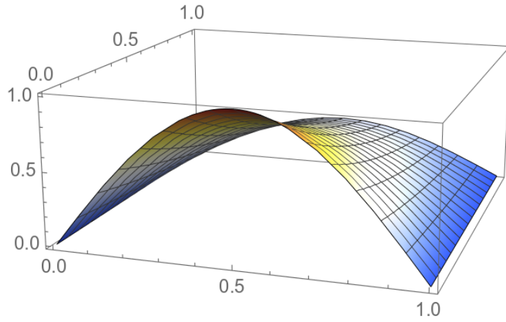
Figure 8: Numerical approximation of the parabolic PDE
