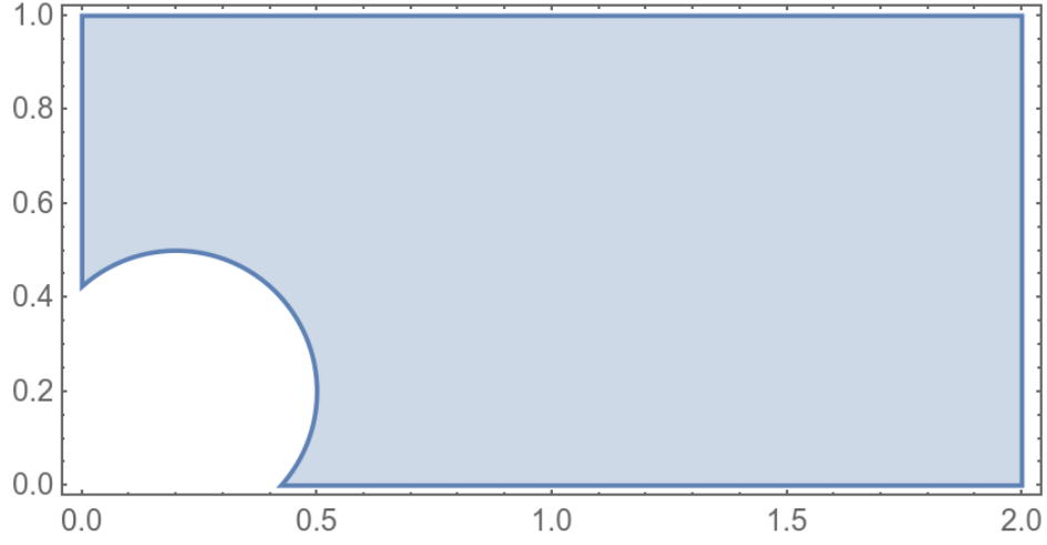
Figure 3: Region excluding the points described by 31
