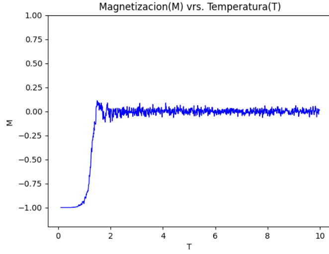
Figure 8: Magnetization versus temperature
