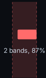
B4 649-680 nm
