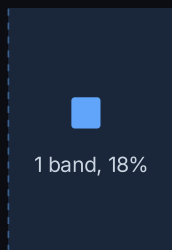
B2 459-525 nm
