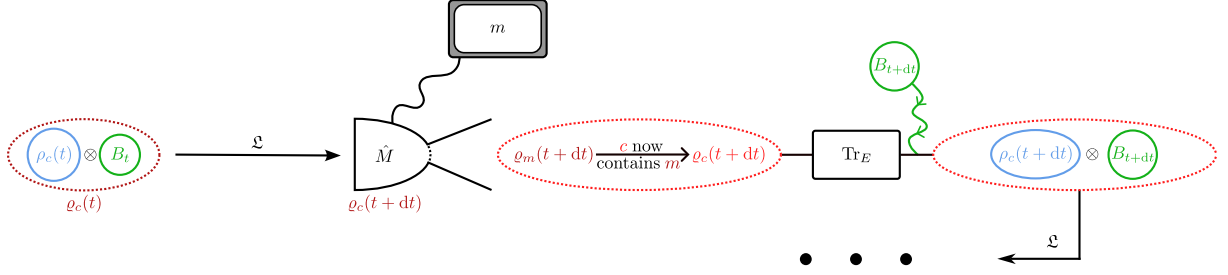
Figure 1: Scheme of continuous monitoring. In the first place the total system evolves from time t to t + dt according to the Lindblad master equation (denoted as \mathfrak{L} ). We then measure the total state according to the observable \hat{M} we denote the outcome as m . We could label the total state with m , however we only specify that the state is conditional with c . Then, by tracing out the environment, we find \rho_c(t + dt) but it instantaneously couples with the next temporal mode B_{t+dt} . This process is repeated until the end of the monitoring.
