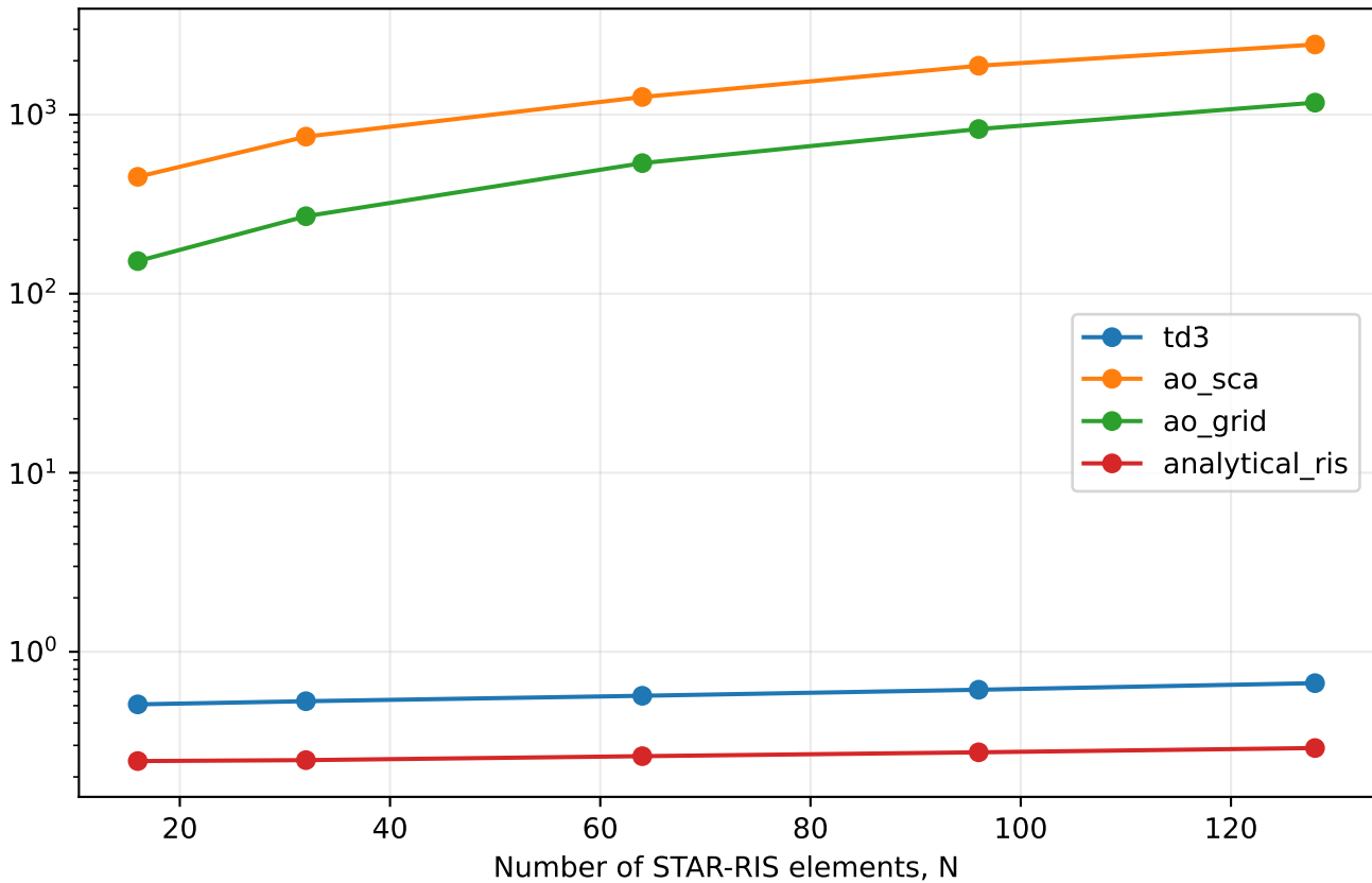
Mean end-to-end CPU latency (ms)
