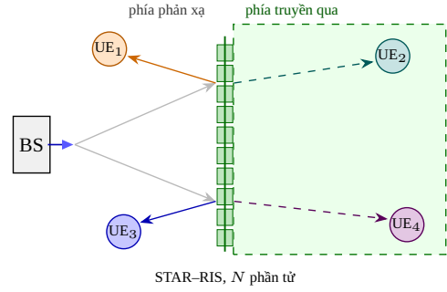
(b) STAR-RIS
