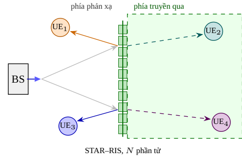
(b) STAR-RIS
