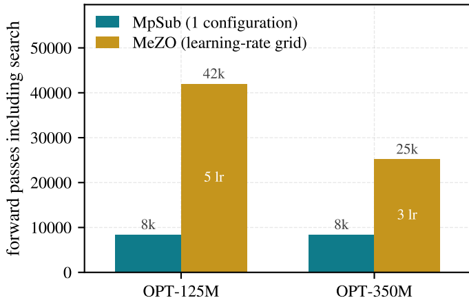
Cost of reaching it
