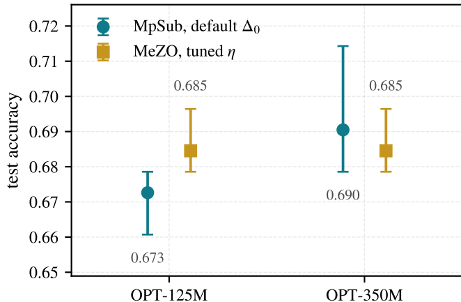
Accuracy at matched compute
