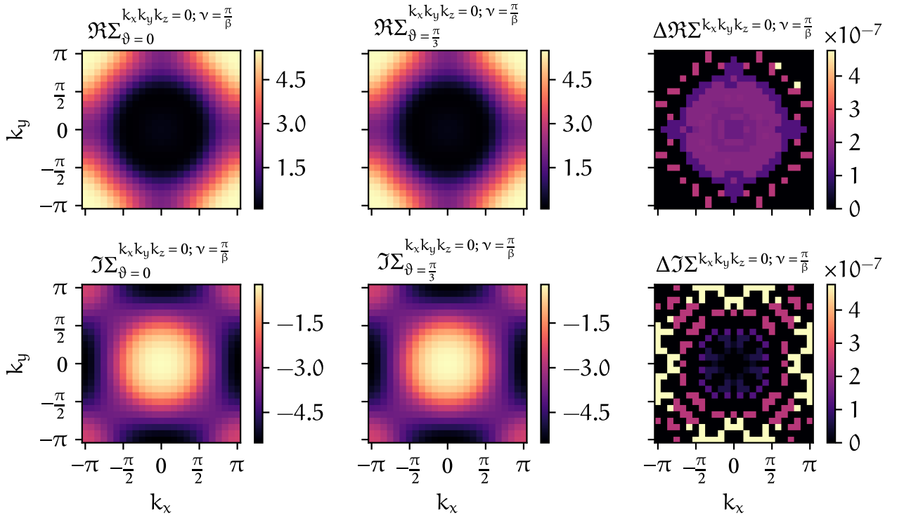
FIGURE 5.12 – Differences (last column) between the two-band calculation without a rotation ( \vartheta = 0 , first column) and a calculation, where the input data was rotated before the D \Gamma A calculation and subsequently rotated back by a factor of \vartheta = \frac{\pi}{3} (second column) for both the real and imaginary part of the self-energy (first and second row, respectively).
