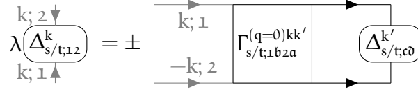
FIGURE 4.2 – Linearized Eliashberg equation for vanishing transfer frequency q = 0 , see Eq. (4.41).
