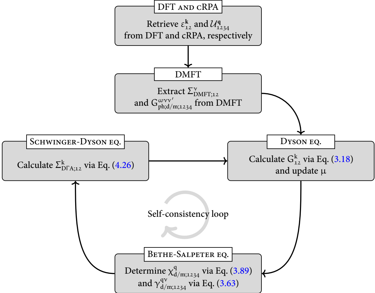
FIGURE 4.1 – This flowchart shows the D\Gamma A self-consistency cycle. The first box is concerned with the bandstructure and interaction calculations using DFT and/or cRPA. The next box denotes the DMFT calculation which is performed using the previously calculated quantities. From the converged DMFT calculation we extract the DMFT self-energy and local two-particle vertex functions, such as the two-particle Green’s function in the ph and pp-channel. The three boxes below describe the self-consistency cycle of the D\Gamma A approach. The output quantities from DFT/cRPA and DMFT, i.e. all purely local vertex functions and the interaction, are kept constant throughout the D\Gamma A self-consistency cycle.
