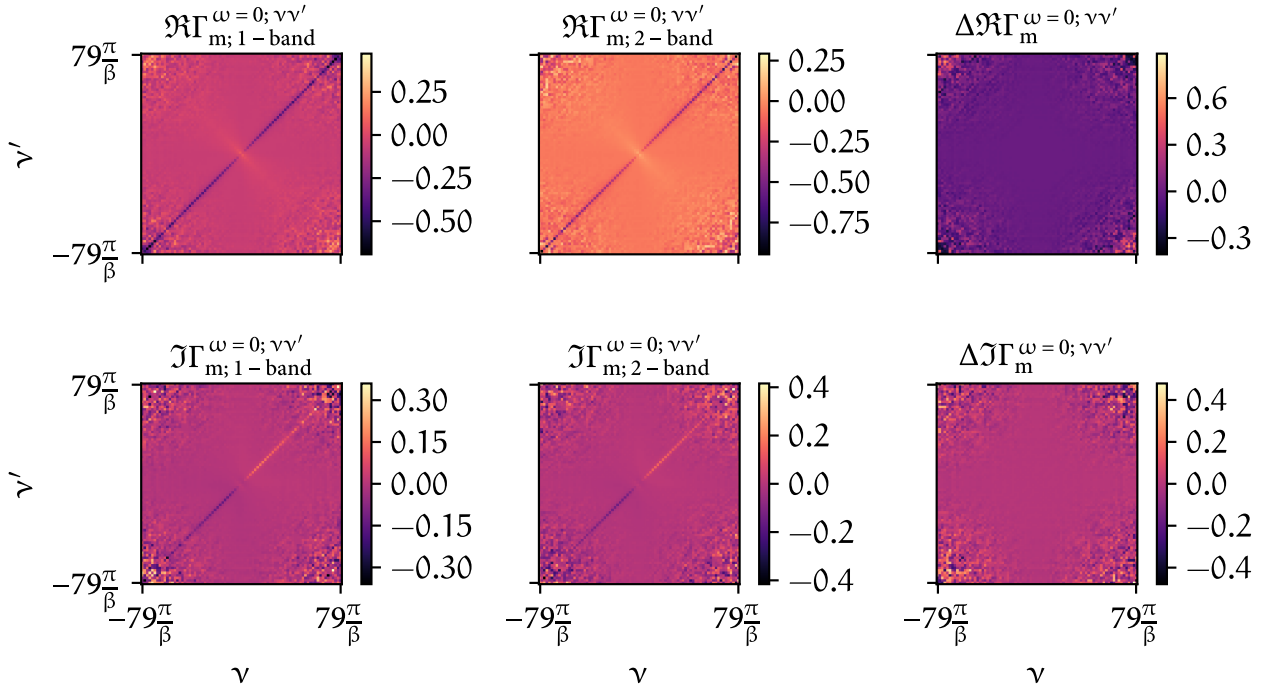
FIGURE 5.10 – Similar to Fig. 5.7 but with a four-times increase in measurement statistics for the one- and two-particle calculations in w2dynamics.
