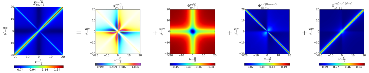
FIGURE 3.14 – Numerical SIAM results for all local vertices contained in the parquet equation Eq. (3.33) for vanishing transfer frequency \Omega = 0 , taken from Ref. [52]. In our convention, \Omega should be replaced by \omega .
