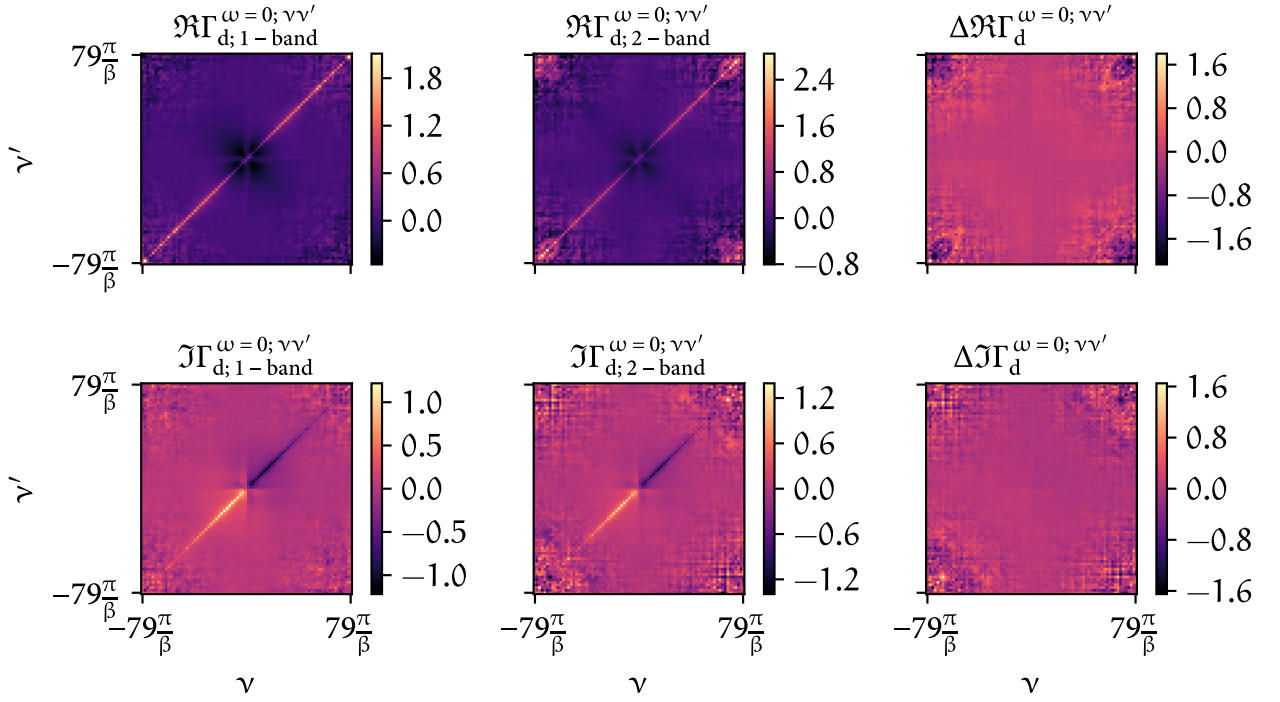
FIGURE 5.6 – Differences (last column) between the real and imaginary part of the local irreducible vertex in the density channel calculated from the one-band dataset (first column) and the fictitious two-band dataset (second column).
