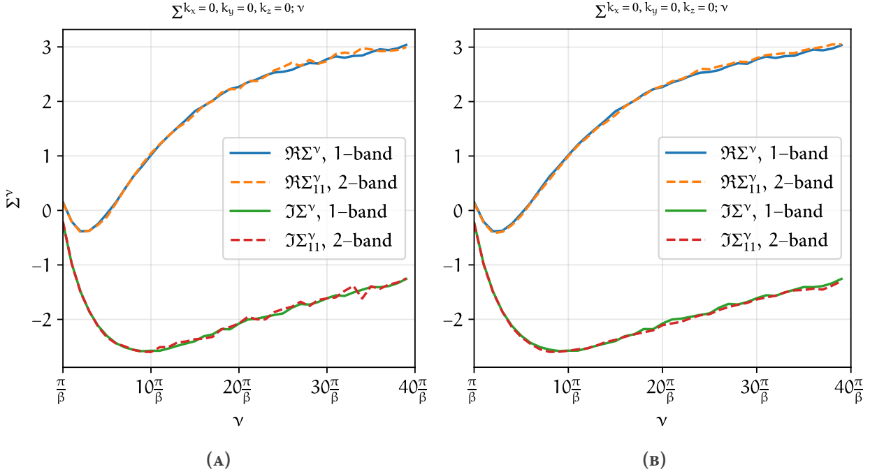
FIGURE 5.11 – Frequency dependence of the real and imaginary part of the self-energy for the single-band and the fictitious two-band dataset. (A) shows the comparison for a lower QMC statistics run for the two-band dataset, whereas (B) for a four-times higher one. The improved behaviour for large frequencies is not surprising, as the increase of QMC measurements mitigates some stochastic noise.
