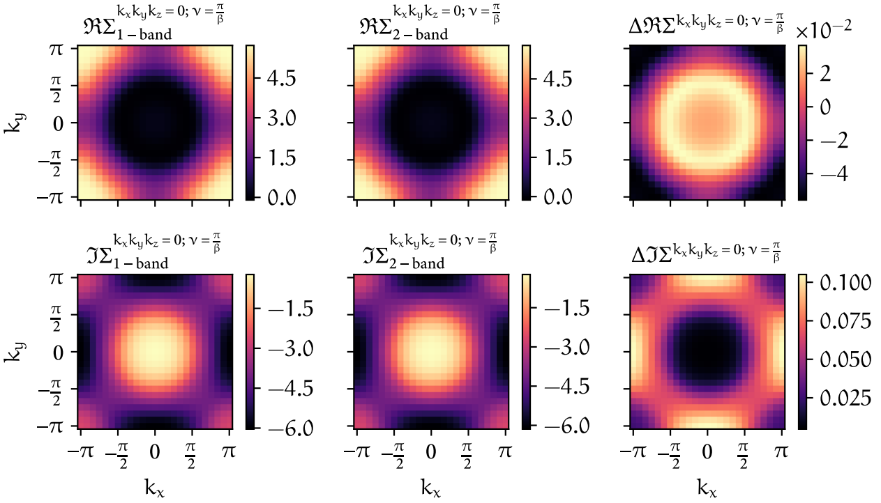
FIGURE 5.8 – Similar to Fig. 5.5 but with a four-times increase in measurement statistics for the one- and two-particle calculations in w2dynamics.
