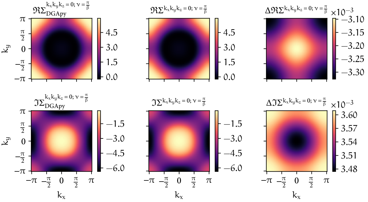
FIGURE 5.2 – Analogous to Fig. 5.1, but with the double-counting kernel of Eq. (4.29).
