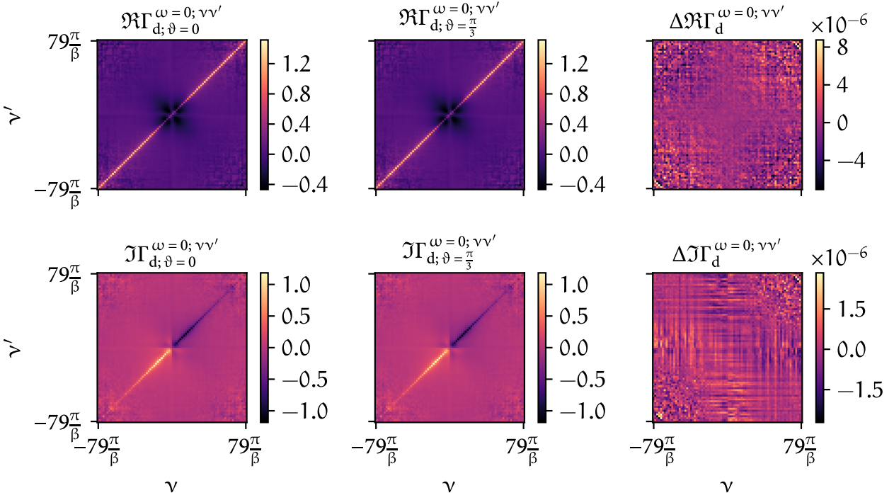
FIGURE 5.13 – Differences (last column) between the two-band calculation without a rotation ( \vartheta = 0 , first column) and a calculation, where the input data was rotated before the D \Gamma A calculation and subsequently rotated back by a factor of \vartheta = \pi/3 (second column) for both the real and imaginary part of the local irreducible vertex \Gamma_d^{\omega=0; \nu\nu'} (first and second row, respectively) in the density spin combination.
