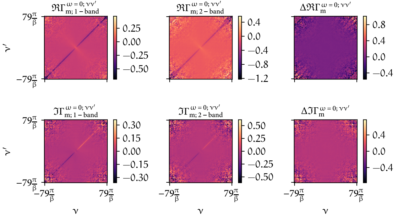
FIGURE 5.7 – Analogous to Fig. 5.6 but for the magnetic spin combination.
