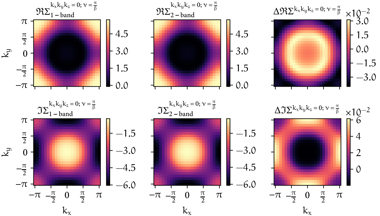
FIGURE 5.5 – Differences between the one-band self-energy (first column) and the first diagonal component of the self-energy (second column) calculated from the fictitious two-band system. The difference between both can be seen in the last column and the rows indicate the real- and imaginary part of all self-energies, respectively.
