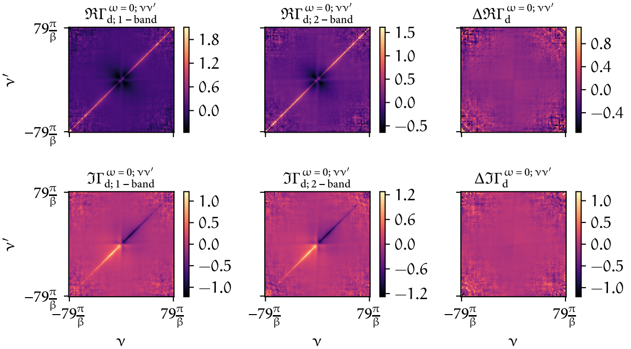
FIGURE 5.9 – Similar to Fig. 5.6 but with a four-times increase in measurement statistics for the one- and two-particle calculations in w2dynamics.
