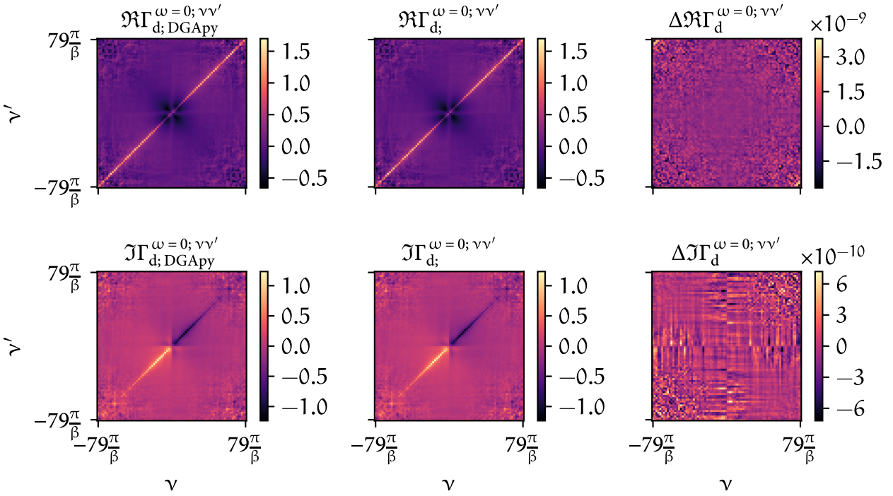
FIGURE 5.3 – Differences (third column) between the real and imaginary part of the local irreducible vertex in the density channel calculated with DGApv (first column) and the new program (second column).
