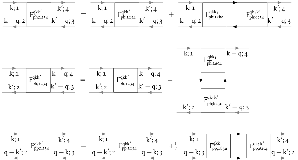
FIGURE 1.10 – Diagrammatic version of the BSE in all three channels for arbitrary spin components, see Eq. (3.48). The lower legs are exchanged in pp-notation, hence their direction is reversed.
