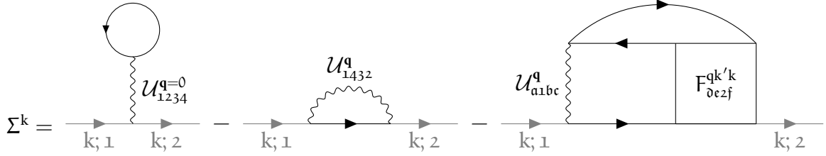
FIGURE 1.12 – Representation of the Schwinger-Dyson equation, see Eq. (3.55).
