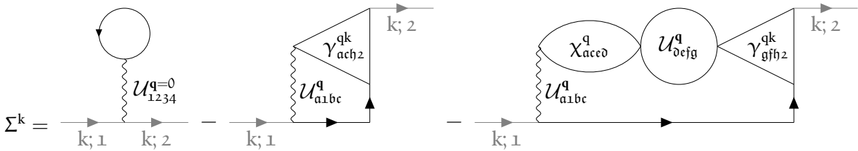
FIGURE 1.14 – Interaction-reducible form of the Schwinger-Dyson equation (3.64) with three-leg vertices.
