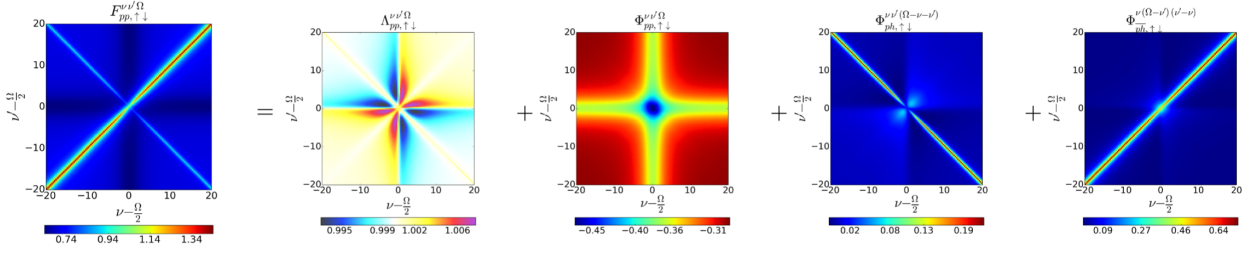
FIGURE 1.15 – Numerical SIAM results for all local vertices contained in the parquet equation Eq. (3.32) for vanishing transfer frequency \Omega = 0 , taken from Ref. [24]. In our convention, \Omega should be replaced by \omega .
