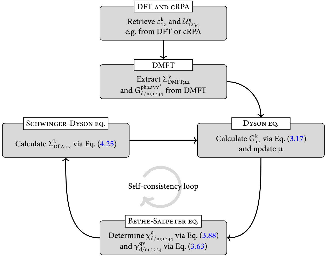
FIGURE 4.1 – This flowchart shows the D \Gamma A self-consistency cycle. The first box is concerned with the bandstructure and interaction calculations which can be obtained from simple model studies or e.g. DFT or cRPA. The next box denotes the DMFT calculation which is performed using the previously acquired bandstructure and interaction. From the converged DMFT calculation we extract the DMFT self-energy and the local two-particle Green’s function. The three boxes below describe the self-consistency cycle of the D \Gamma A approach. The bandstructure, interaction and output quantities from DMFT, i.e. all purely local (ir-)reducible vertex functions are kept constant throughout the whole D \Gamma A self-consistency cycle.
