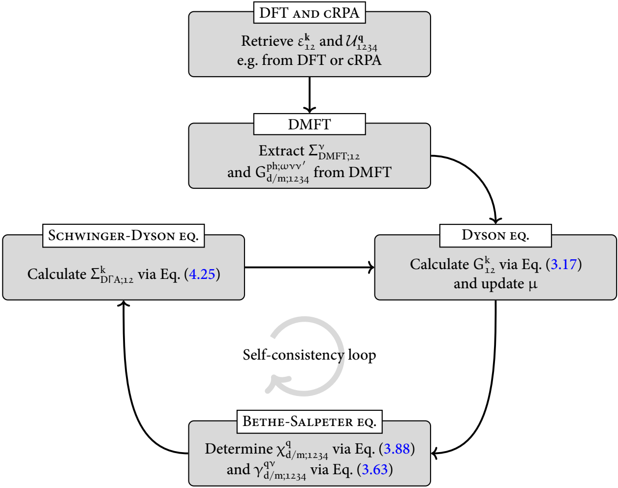
FIGURE 4.1 – This flowchart shows the \text{D}\Gamma\text{A} self-consistency cycle. The first box is concerned with the bandstructure and interaction calculations which can be obtained from simple model studies or e.g. DFT or cRPA. The next box denotes the DMFT calculation which is performed using the previously acquired bandstructure and interaction. From the converged DMFT calculation we extract the DMFT self-energy and the local two-particle Green’s function. The three boxes below describe the self-consistency cycle of the \text{D}\Gamma\text{A} approach. The bandstructure, interaction and output quantities from DMFT, i.e. all purely local (ir-)reducible vertex functions are kept constant throughout the whole \text{D}\Gamma\text{A} self-consistency cycle.
