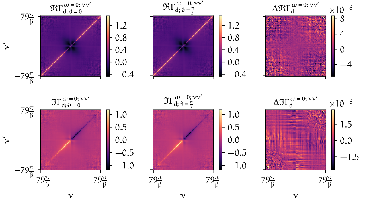
FIGURE 5.13 – Two-band calculation without a rotation ( \vartheta = 0 , first column) and a calculation, where the input data was rotated before the D \Gamma A calculation and subsequently rotated back by a factor of \vartheta = \frac{\pi}{3} (second column) for both the real and imaginary part of the local irreducible vertex \Gamma_d^{\omega=0; \nu\nu'} (first and second row, respectively) in the density spin combination. Their differences are shown in the third column.
