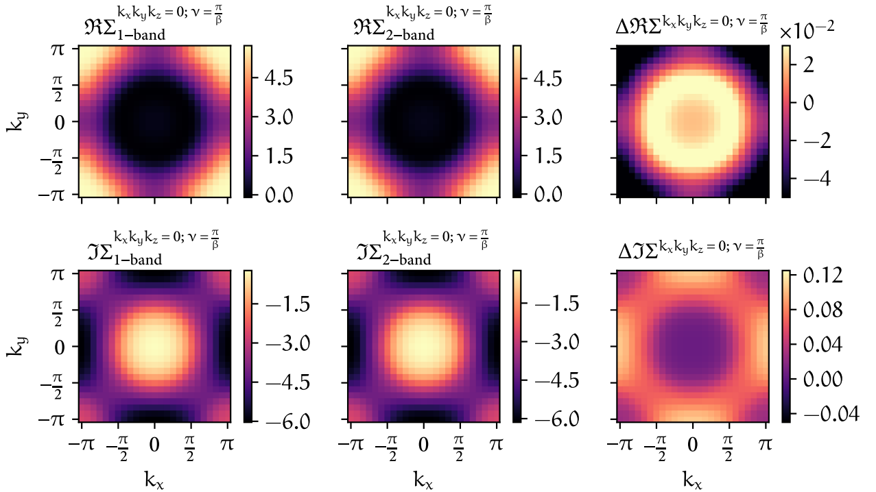
FIGURE 5.5 – One-band self-energy (first column) and the first diagonal component of the self-energy from the artificial two-band system (second column) calculated using the inputs from separate w2dynamics runs. The difference between both can be seen in the last column and the rows indicate the real- and imaginary part of all self-energies, respectively.
