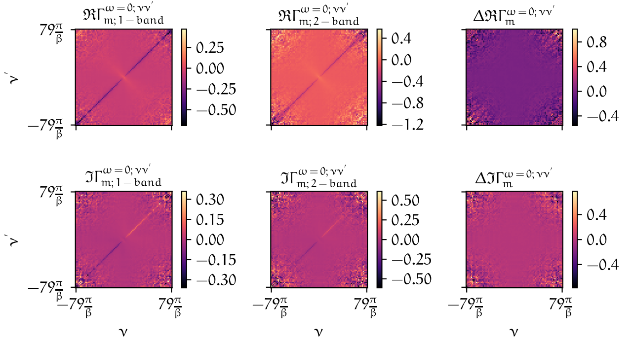
FIGURE 1.7 – Analogous to Fig. 1.3 but for the magnetic spin combination.
