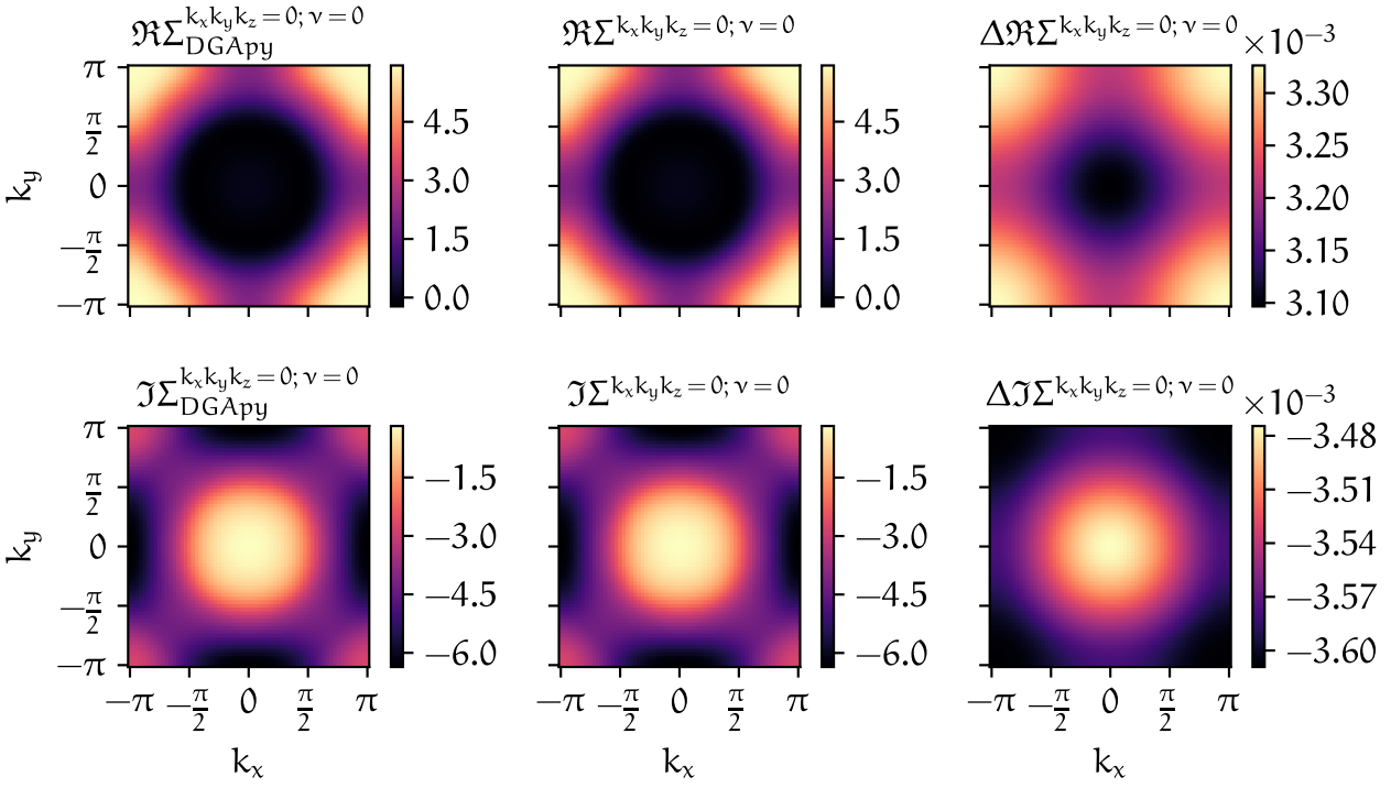
FIGURE 4.2 – Analogous to Fig. 4.1, but with the double-counting kernel of Eq. (3.124).
