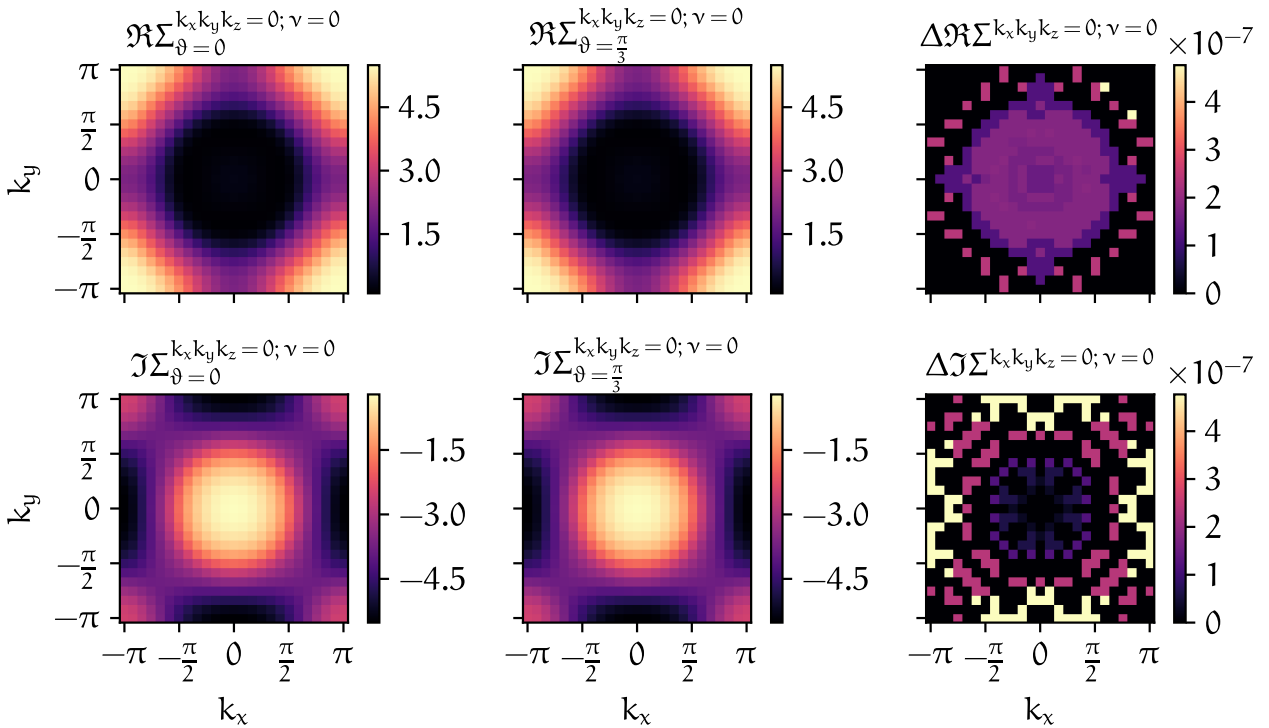
FIGURE 4.8 – Differences (last column) between the two-band calculation without a rotation ( \vartheta = 0 , first column) and a calculation, where the input data was rotated before the D \Gamma A calculation and subsequently rotated back by a factor of \vartheta = \frac{\pi}{3} (second column) for both the real and imaginary part of the self-energy (first and second row, respectively).
