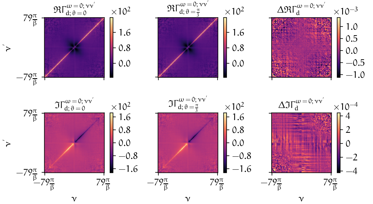
FIGURE 4.9 – Differences (last column) between the two-band calculation without a rotation ( \vartheta = 0 , first column) and a calculation, where the input data was rotated before the D \Gamma A calculation and subsequently rotated back by a factor of \vartheta = \frac{\pi}{3} (second column) for both the real and imaginary part of the local irreducible vertex \Gamma_d^{\omega=0; \nu\nu'} (first and second row, respectively) in the density spin combination.
