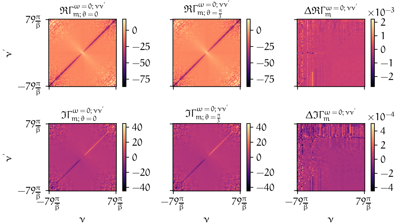
FIGURE 4.10 – Analogous to Fig. 4.9 but for the magnetic spin combination.
