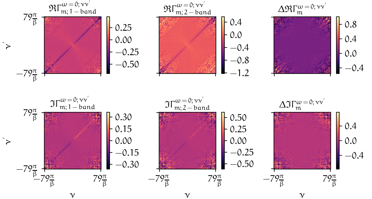
FIGURE 4.7 – Analogous to Fig. 4.3 but for the magnetic spin combination.
