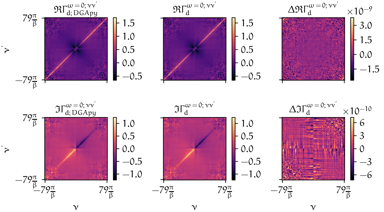
FIGURE 4.3 – Differences (third column) between the real and imaginary part of the local irreducible vertex in the density channel calculated with DGApy (first column) and the new program (second column).
