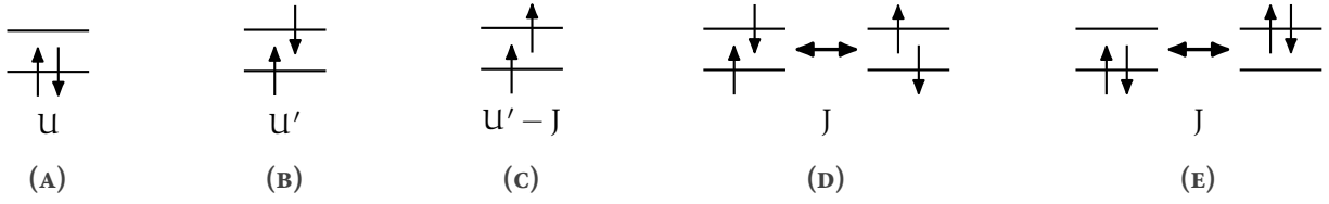
FIGURE 1.2 – Kanamori parameters U , U' and J as described in the text: (A) intra-orbital Coulomb interaction, (B)-(C) inter-orbital Coulomb interaction, (D) spin-flip of an electron pair and (E) pair hopping.
