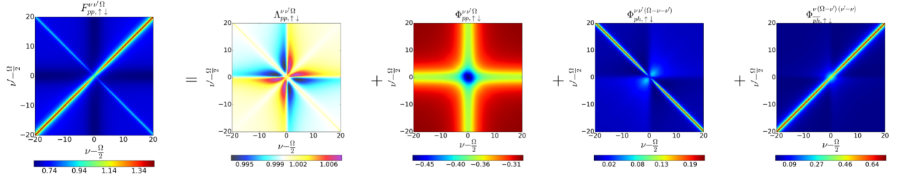
FIGURE 3.14 – Numerical SIAM results for all local vertices contained in the parquet equation Eq. (3.33) for vanishing transfer frequency \Omega = 0 , taken from Ref. [45]. In our convention, \Omega should be replaced by \omega .
