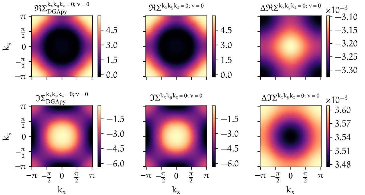
FIGURE 4.2 – Analogous to Fig. 4.1, but with the double-counting kernel of Eq. (3.124).
