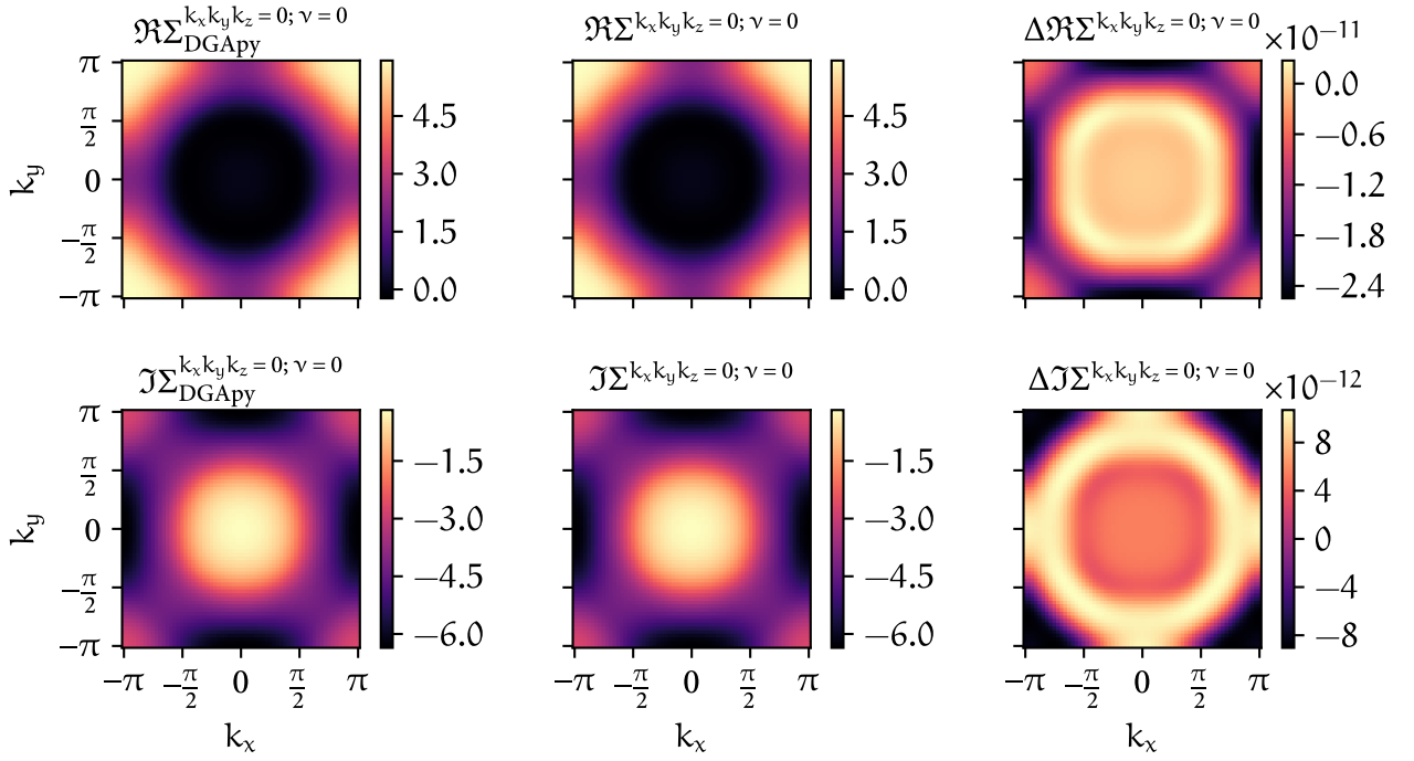
FIGURE 4.1 – Difference between the one-band self-energy of DGApy (first column) and the current implementation with the double-counting kernel of Eq. (4.2) (second column) for k_z = 0 and v = 0 . The difference between both, i.e. \Delta \Sigma = \Sigma_{\text{DGApy}} - \Sigma , can be seen in the last column. The rows indicate the real- and imaginary part of all self-energies, respectively.
