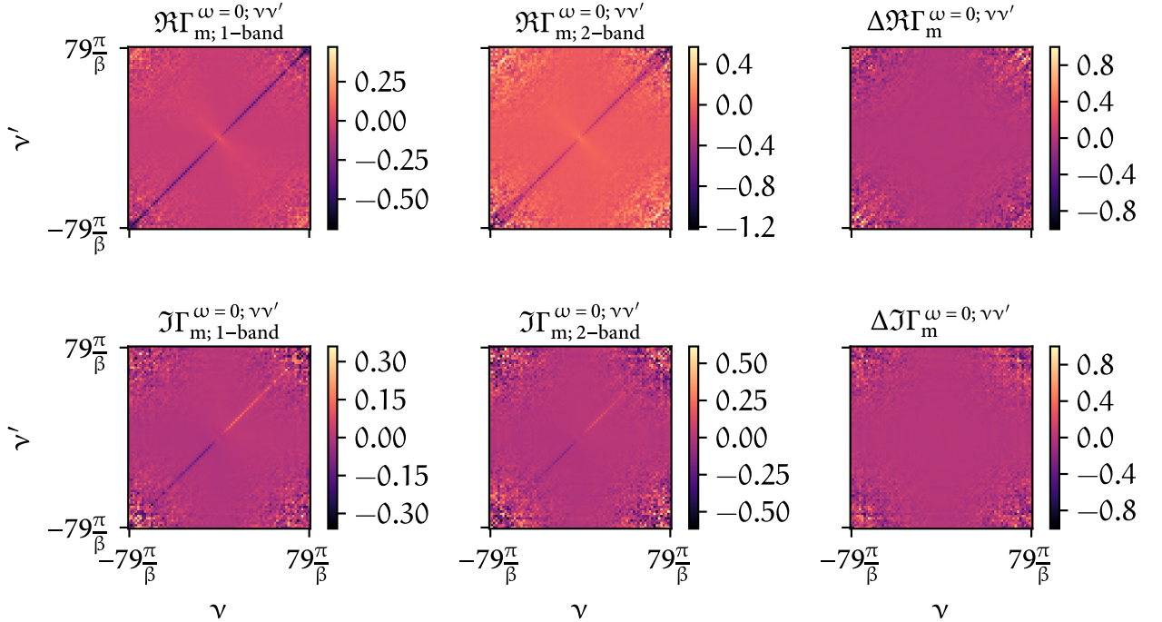
FIGURE 1.7 – Analogous to Fig. ?? but for the magnetic spin combination.
