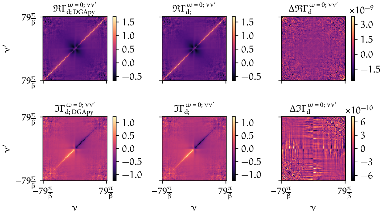
FIGURE 1.3 – Real and imaginary part of the local irreducible vertex in the density channel calculated with DGApY (first column) and moLDGA (second column). Their differences can be seen in the third column.
