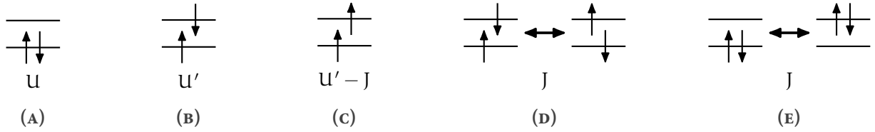
FIGURE 1.2 – Kanamori parameters U , U' and J as described in the text: (??) intra-orbital Coulomb interaction, (??)-(??) inter-orbital Coulomb interaction, (??) spin-flip of an electron pair and (??) pair hopping. Adapted from Ref. [Galler2018] to match the style of this thesis.
