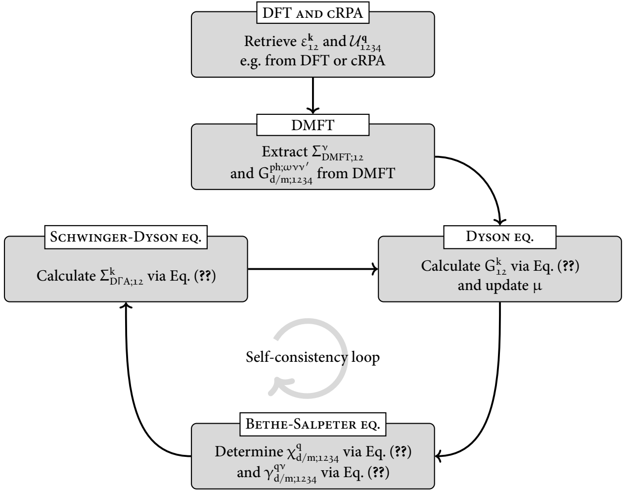
FIGURE 1.1 – Flowchart of the D \Gamma A self-consistency cycle. The first box is concerned with the bandstructure and interaction calculations which can be obtained from simple model studies or for actual materials from DFT and cRPA. The next box denotes the DMFT calculation which is performed using the previously acquired bandstructure and interaction. From the converged DMFT calculation we extract the DMFT self-energy and the local two-particle Green’s function. The three boxes below describe the self-consistency cycle of the D \Gamma A approach. The bandstructure, interaction and output quantities from DMFT, i.e. all purely local (ir-)reducible vertex functions are kept constant throughout the whole D \Gamma A self-consistency cycle.
