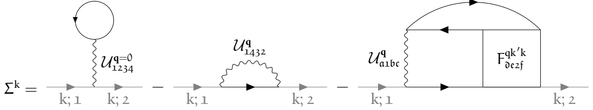
FIGURE 1.12 – Representation of the Schwinger-Dyson equation, see Eq. (1.55).
