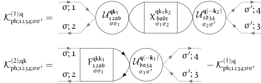
FIGURE 1.16 – Diagrammatic version of the kernel-1 and kernel-2 functions of Eq. (1.69) and Eq. (1.71).
