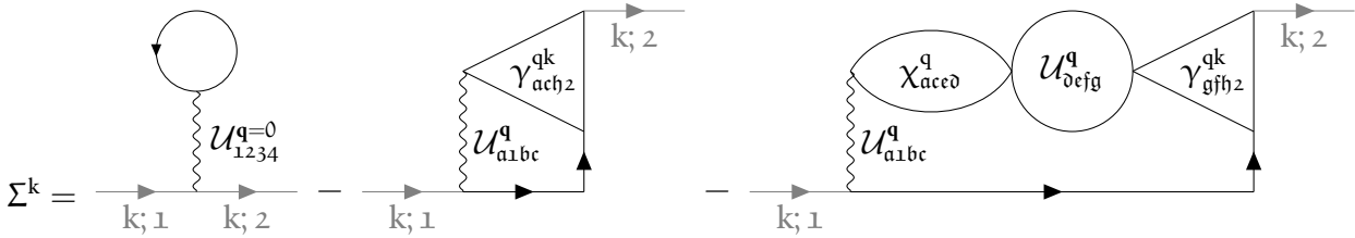
FIGURE 1.14 – Interaction-reducible form of the Schwinger-Dyson equation (1.64) with three-leg vertices.
