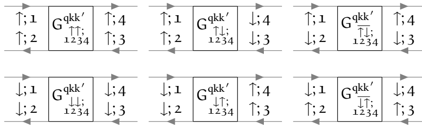
FIGURE 1.4 – In the absence of spin-orbit coupling, these are the only non-vanishing spin combinations of the two-particle Green's function.
