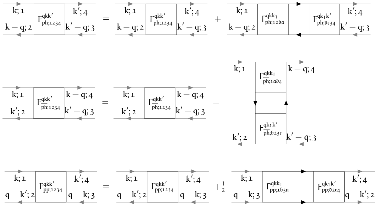
FIGURE 1.10 – Diagrammatic version of the BSE in all three channels for arbitrary spin components, see Eq. (1.48). The lower legs are exchanged in pp-notation, hence their direction is reversed.
