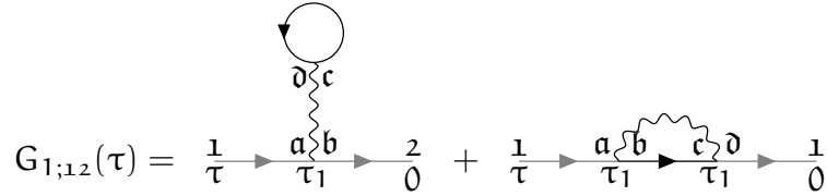
FIGURE 1.2 – First order diagrams for the single-particle Green's function. The corresponding diagrams are coined the Hartree- and the Fock-term, respectively. As the name suggests, taking only these two diagrams as the whole perturbation expansion leads to the Hartree-Fock approximation, formulated as a diagrammatic theory.
