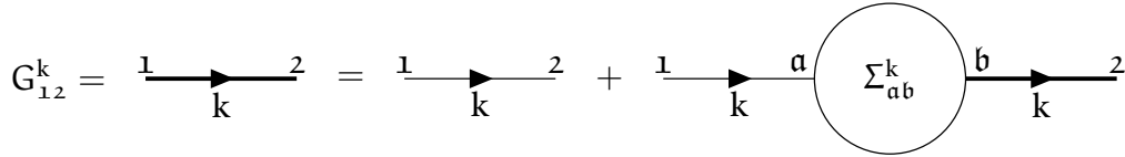
FIGURE 1.3 – Diagrammatic representation of Eq. (1.17). The full Green's function G_{12}^k is drawn as a thick black line.
