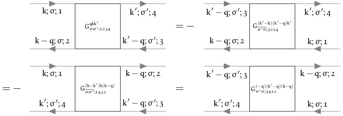
FIGURE 1.5 – Diagrammatic representation of the crossing symmetry relations in order of Eq. (1.26a) - Eq. (1.26c).
