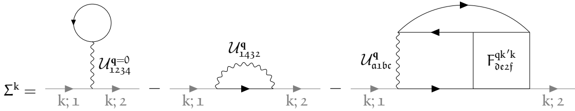
FIGURE 3.11 – Representation of the Schwinger-Dyson equation, see Eq. (3.55).
