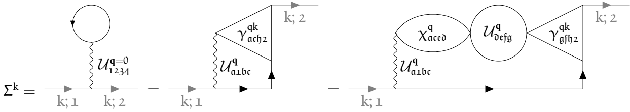
FIGURE 3.13 – Interaction-reducible form of the Schwinger-Dyson equation (3.63) with three-leg vertices.
