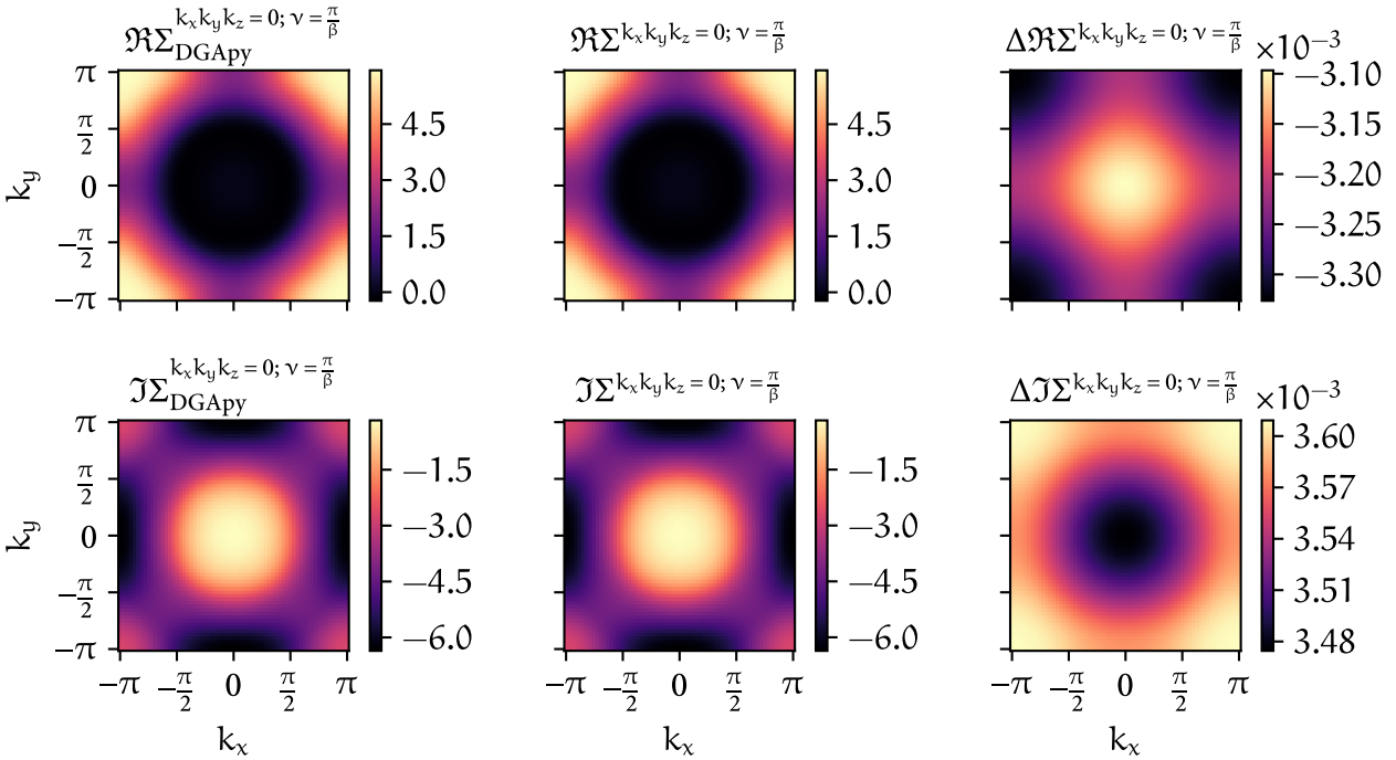
FIGURE 5.2 – Analogous to Fig. 5.1, but with the double-counting kernel of Eq. (4.28).
