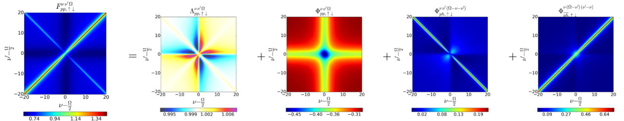
FIGURE 3.15 – Numerical SIAM results for all local vertices contained in the parquet equation Eq. (3.32) for vanishing transfer frequency \Omega = 0 , taken from Ref. [55]. In our convention, \Omega should be replaced by \omega .
