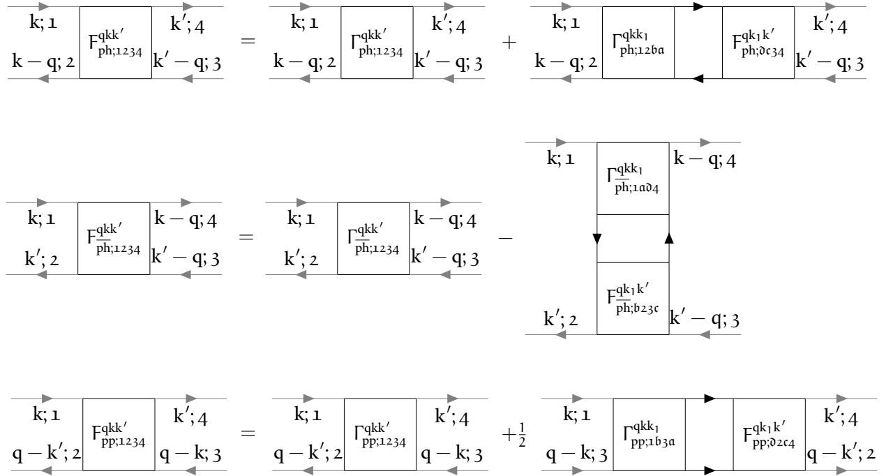
FIGURE 3.10 – Diagrammatic version of the BSE in all three channels for arbitrary spin components, see Eq. (3.48). The lower legs are exchanged in pp-notation, hence their direction is reversed.
