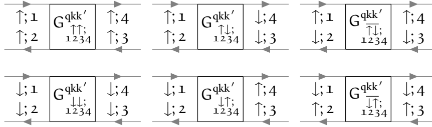
FIGURE 3.4 – In the case of absent spin-orbit coupling, these are the only non-vanishing spin combinations of the two-particle Green's function.
