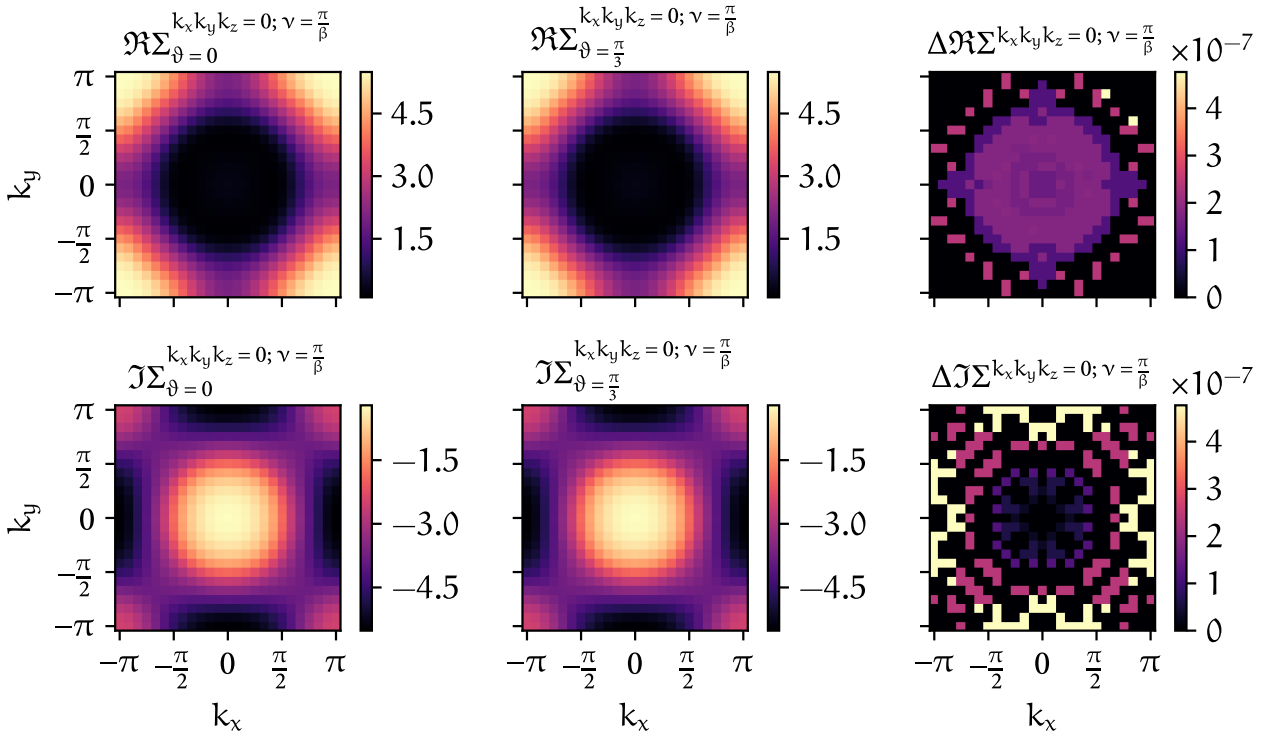
FIGURE 5.12 – Two-band calculation without a rotation ( \vartheta = 0 , first column) and a calculation, where the input data was rotated before the D \Gamma A calculation and subsequently rotated back by a factor of \vartheta = \frac{\pi}{3} (second column) for both the real and imaginary part of the self-energy (first and second row, respectively). Their differences are shown in the third column.
