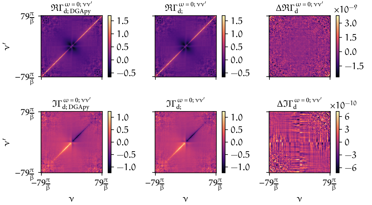
FIGURE 5.3 – Real and imaginary part of the local irreducible vertex in the density channel calculated with DGApY (first column) and the new program (second column). Their differences can be seen in the third column.
