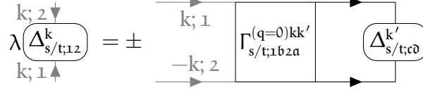
FIGURE 1.2 – Linearized Eliashberg equation for vanishing transfer frequency q = 0 , see Eq. (4.40).
