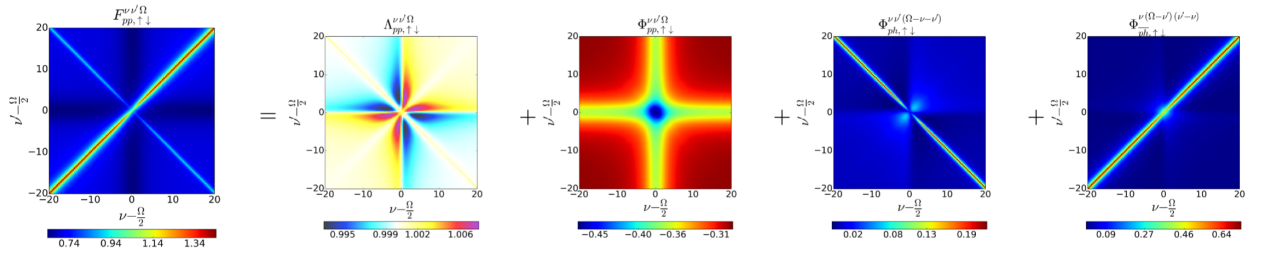
FIGURE 1.14 – Numerical SIAM results for all local vertices contained in the parquet equation Eq. (3.32) for vanishing transfer frequency \Omega = 0 , taken from Ref. [Wentzell2020]. In our convention, \Omega should be replaced by \omega .
