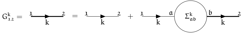
FIGURE 1.3 – Diagrammatic representation of Eq. (3.17). The full Green's function G_{12}^k is drawn as a thick black line.
