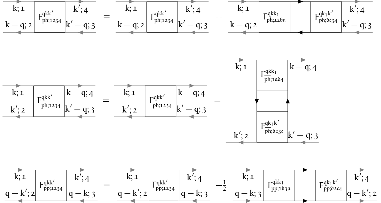
FIGURE 1.10 – Diagrammatic version of the BSE in all three channels for arbitrary spin components, see Eq. (3.48). The lower legs are exchanged in pp-notation, hence their direction is reversed.
