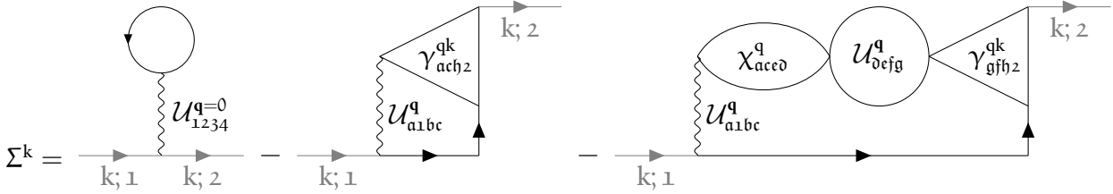
FIGURE 1.13 – Interaction-reducible form of the Schwinger-Dyson equation (3.63) with three-leg vertices.
