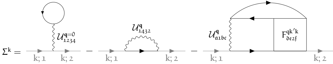
FIGURE 1.11 – Representation of the Schwinger-Dyson equation, see Eq. (3.55).
