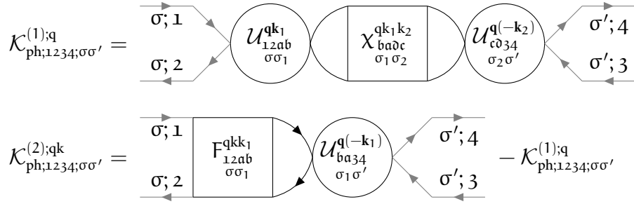
FIGURE 1.16 – Diagrammatic version of the kernel-1 and kernel-2 functions of Eq. (3.69) and Eq. (3.71).
