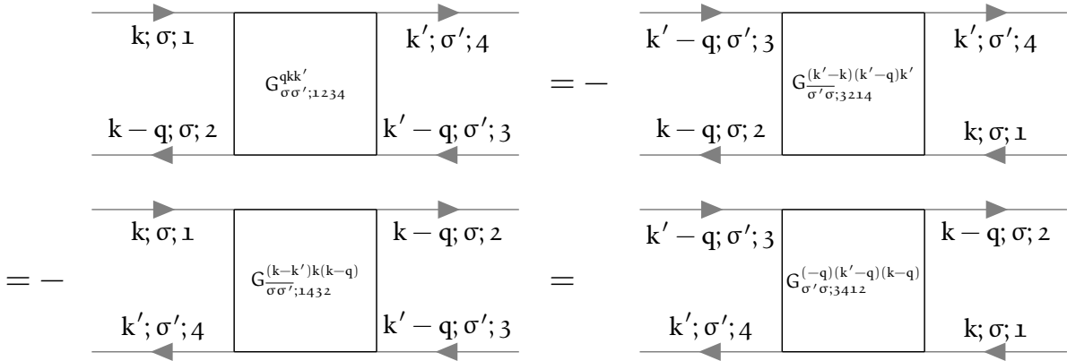
FIGURE 1.5 – Diagrammatic representation of the crossing symmetry relations in order of Eq. (3.26a) - Eq. (3.26c).
