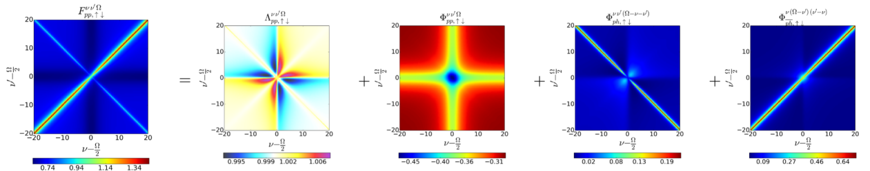
FIGURE 3.15 – Numerical SIAM results for all local vertices contained in the parquet equation Eq. (3.32) for vanishing transfer frequency \Omega = 0 , taken from Ref. [55]. In our convention, \Omega should be replaced by \omega .
