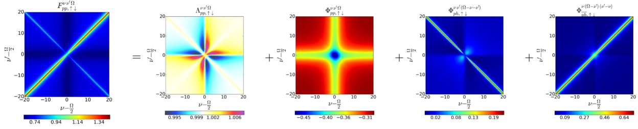
FIGURE 1.15 – Numerical SIAM results for all local vertices contained in the parquet equation Eq. (1.32) for vanishing transfer frequency \Omega = 0 , taken from Ref. [Wentzell2020]. In our convention, \Omega should be replaced by \omega .
