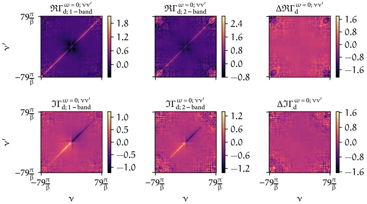
FIGURE 5.6 – Real and imaginary part of the local irreducible vertex in the density channel calculated from the one-band dataset (first column) and the artificial two-band dataset (second column). Their differences are shown in the third column.
