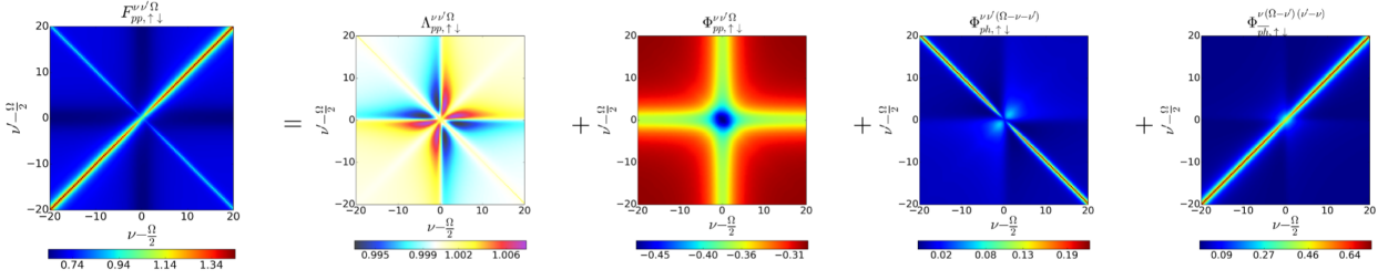
FIGURE 3.15 – Numerical SIAM results for all local vertices contained in the parquet equation Eq. (3.32) for vanishing transfer frequency \Omega = 0 , taken from Ref. [56]. In our convention, \Omega should be replaced by \omega .
