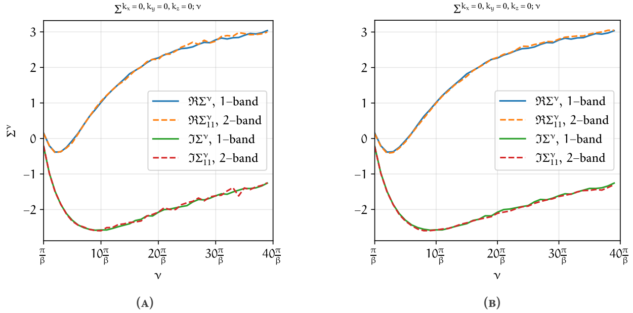
FIGURE 5.11 – Frequency dependence of the real and imaginary part of the self-energy for the single-band and the artificial two-band dataset. (A) shows the comparison for a lower QMC measurement statistics run for the two-band dataset, whereas (B) for a four-times higher number of QMC measurements. The improved behaviour for large frequencies is not surprising, as the increase of QMC measurements mitigates noise.
