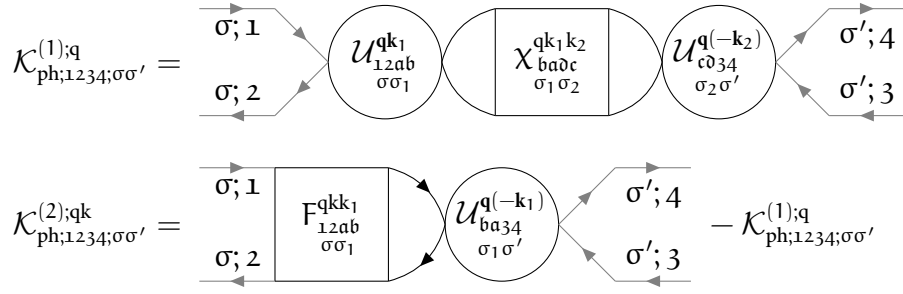
FIGURE 3.16 – Diagrammatic version of the kernel-1 and kernel-2 functions of Eq. (3.69) and Eq. (3.71).
