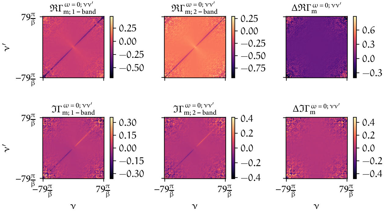
FIGURE 5.10 – Similar to Fig. 5.7 but this time the number of measurement statistics for QMC for the one- and two-particle calculations in w2dynamics were increased by a factor of four.
