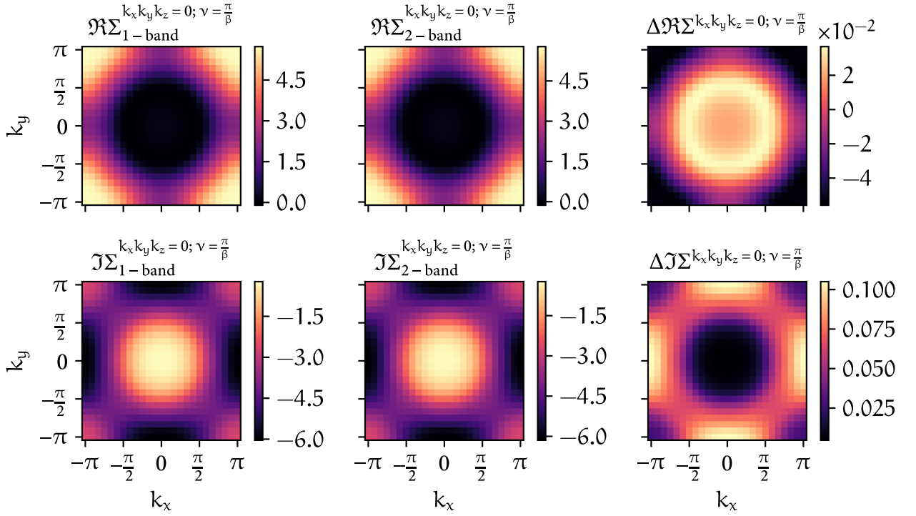
FIGURE 5.8 – Similar to Fig. 5.5 but this time the number of measurement statistics for QMC for the one- and two-particle calculations in w2dynamics were increased by a factor of four.
