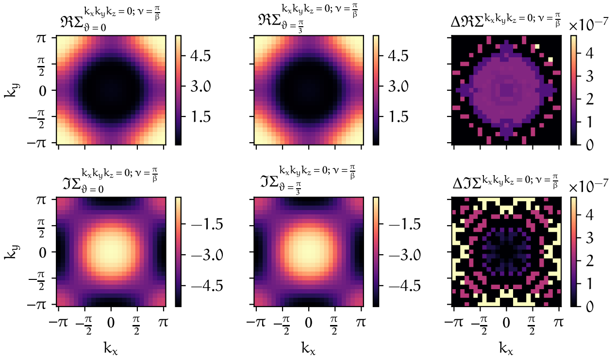
FIGURE 5.12 – Two-band calculation without a rotation ( \vartheta = 0 , first column) and a calculation, where the input data was rotated before the D\Gamma A calculation and subsequently rotated back by a factor of \vartheta = \frac{\pi}{3} (second column) for both the real and imaginary part of the self-energy (first and second row, respectively). Their differences are shown in the third column.
