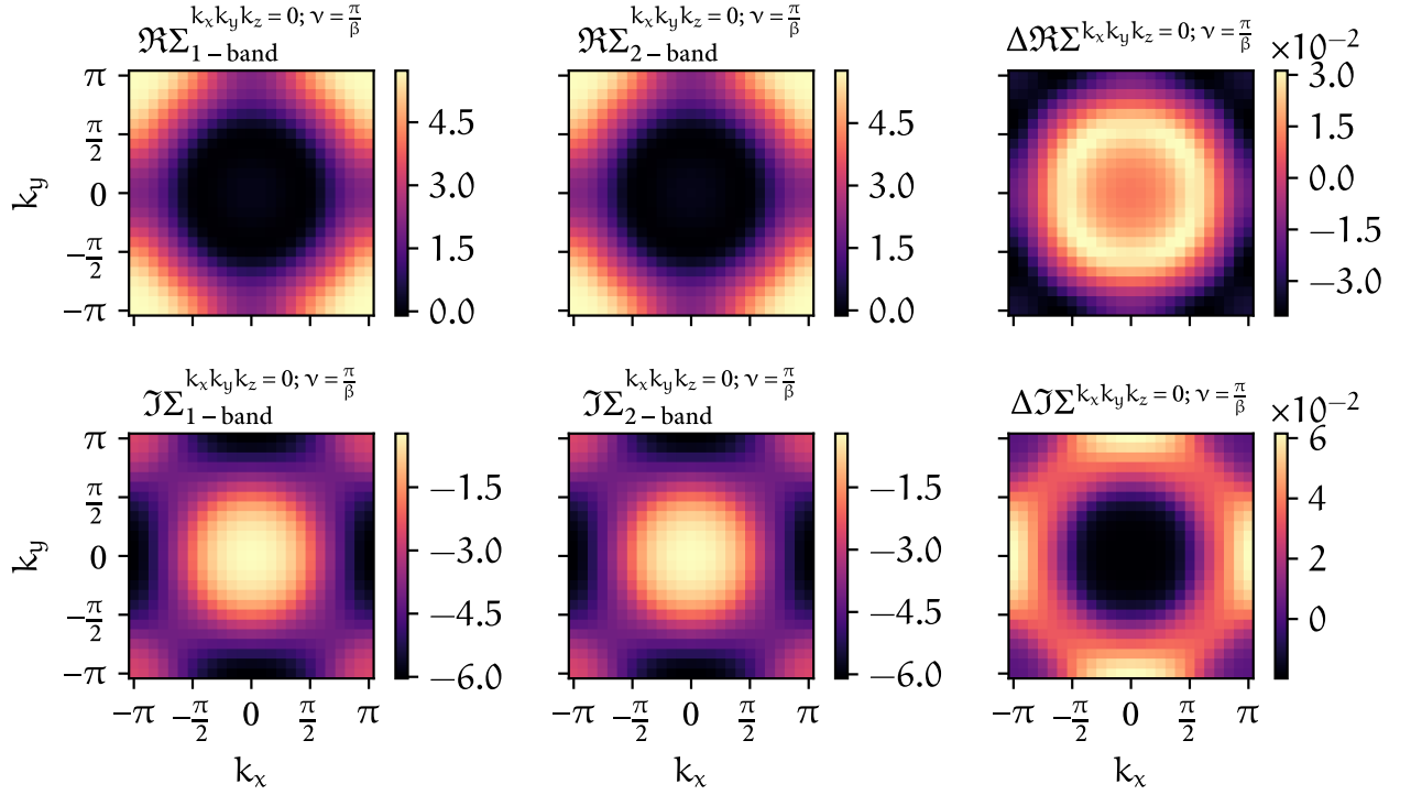
FIGURE 5.5 – One-band self-energy (first column) and the first diagonal component of the self-energy calculated from the artificial two-band system (second column). The difference between both can be seen in the last column and the rows indicate the real- and imaginary part of all self-energies, respectively.
