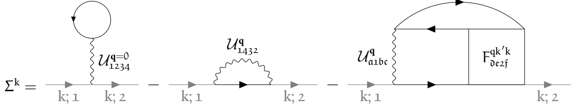
FIGURE 3.12 – Representation of the Schwinger-Dyson equation, see Eq. (3.55).
