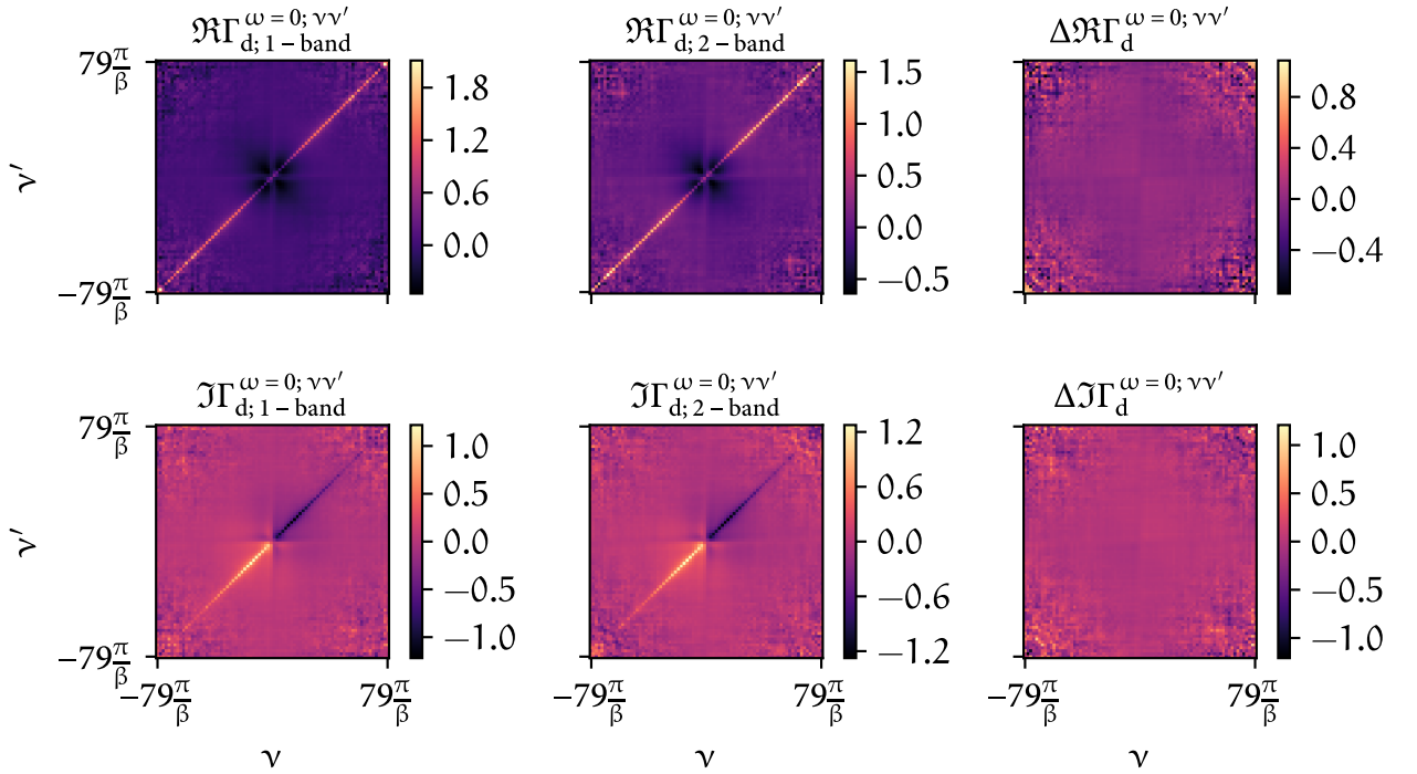
FIGURE 5.9 – Similar to Fig. 5.6 but this time the number of measurement statistics for QMC for the one- and two-particle calculations in w2dynamics were increased by a factor of four.
