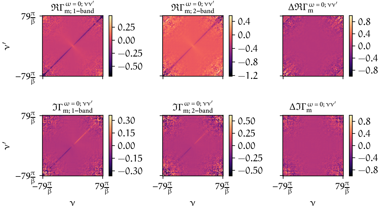
FIGURE 1.7 – Analogous to Fig. ?? but for the magnetic spin combination.
