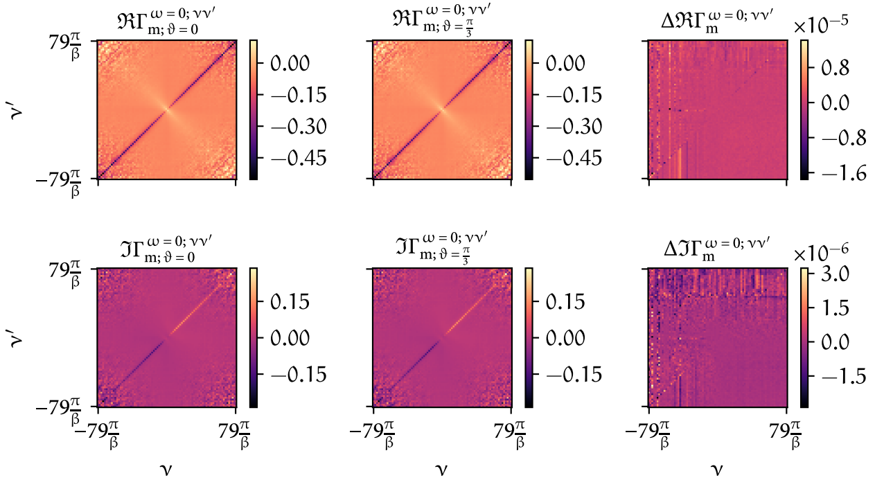
FIGURE 1.14 – Analogous to Fig. ?? but for the magnetic spin combination.
