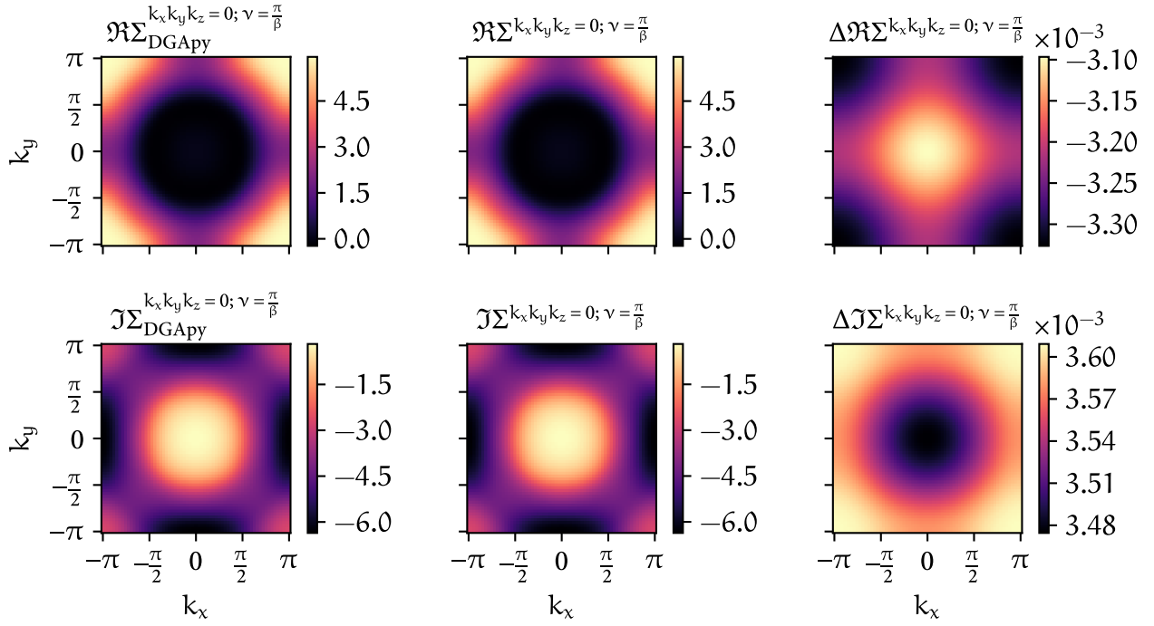
FIGURE 1.2 – Analogous to Fig. ??, but with the double-counting kernel of Eq. (??) applied for moLDGA (second column).
