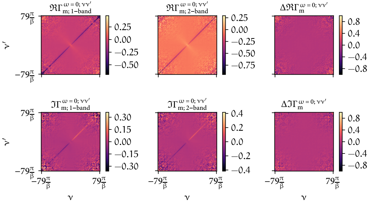
FIGURE 1.10 – Similar to Fig. ?? but this time the number of QMC measurements for the one- and two-particle calculations in w2dynamics were increased by a factor of four.
