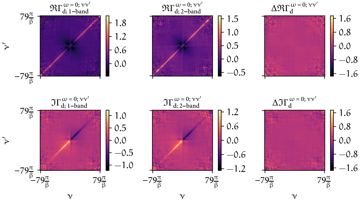
FIGURE 1.9 – Similar to Fig. ?? but this time the number of QMC measurements for the one- and two-particle calculations in w2dynamics were increased by a factor of four.
