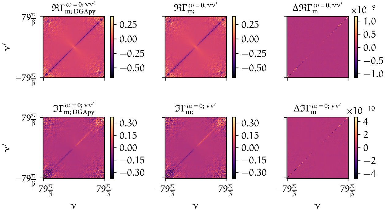
FIGURE 1.4 – Analogous to Fig. ?? but for the magnetic spin combination.
