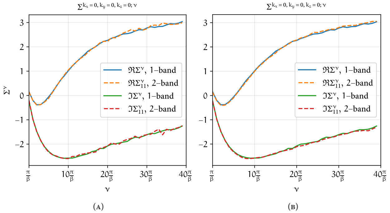
FIGURE 1.11 – Frequency dependence of the real and imaginary part of the self-energy for the single-band and the artificial two-band dataset, and for the \Gamma = (0, 0, 0) point. (??) shows the comparison for a lower QMC measurement statistics run for the two-band dataset, whereas (??) for a four-times higher number of QMC measurements. The improved behavior for large frequencies is not surprising, as the increased number of QMC measurements reduces noise.
