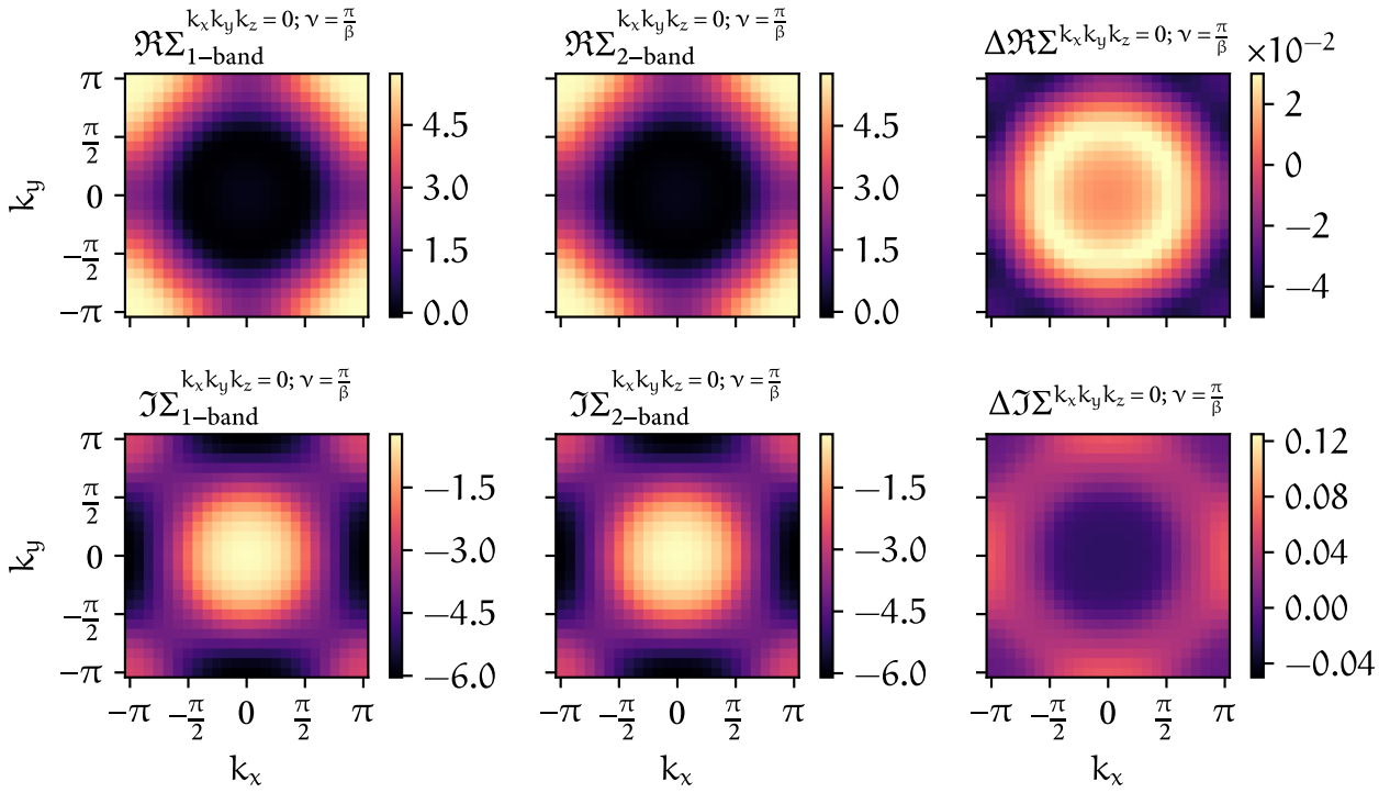
FIGURE 1.8 – Similar to Fig. ?? but this time the number of QMC measurements for the one- and two-particle calculations in w2dynamics were increased by a factor of four.
