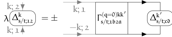
FIGURE 4.2 – Linearized Eliashberg equation for vanishing transfer frequency q = 0 , see Eq. (4.40).
