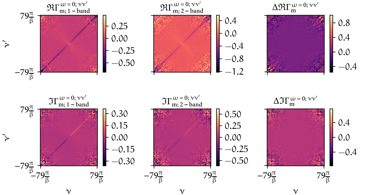
FIGURE 4.7 – Analogous to Fig. 4.6 but for the magnetic spin combination.
