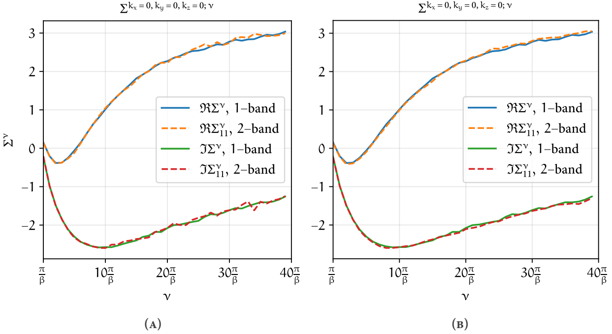
FIGURE 4.11 – Frequency dependence of the real and imaginary part of the self-energy for the single-band and the fictitious two-band dataset. (A) shows the comparison for a lower QMC statistics run for the two-band dataset, whereas (B) for a four-times higher one. The improved behaviour for large frequencies is not surprising, as the increase of QMC measurements mitigates some stochastic noise.
