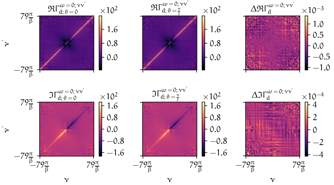
FIGURE 1.6 – Differences (third column) between the two-band calculation without a rotation ( \vartheta = 0 , first column) and a calculation, where the input data was rotated before the D \Gamma A calculation and subsequently rotated back by a factor of \vartheta = \pi/3 (second column) for both the real and imaginary part of the local irreducible vertex \Gamma_d^{\omega=0; \nu\nu'} (first and second row, respectively) in the density spin combination.
