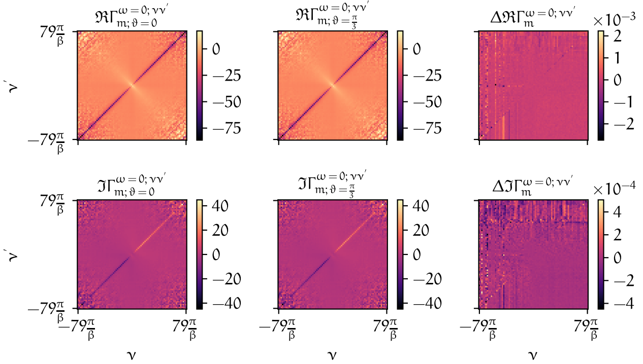
FIGURE 1.7 – Analogous to Fig. 1.6 but for the magnetic spin combination.
