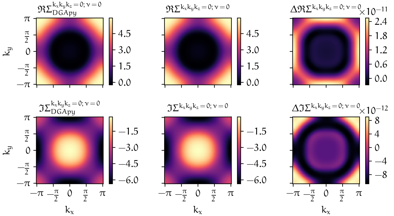
FIGURE 1.1 – Difference between the one-band self-energy of DGApy and the current implementation with the double-counting kernel of Eq. (1.2) for k_z = 0 and v = 0 . The result of DGApy can be seen in the very left column, the result of the current implementation in the second column. The difference between both, i.e. \Delta\Sigma = \Sigma_{\text{DGApy}} - \Sigma , can be seen in the last column. The rows indicate the real- and imaginary part of all self-energies, respectively.
