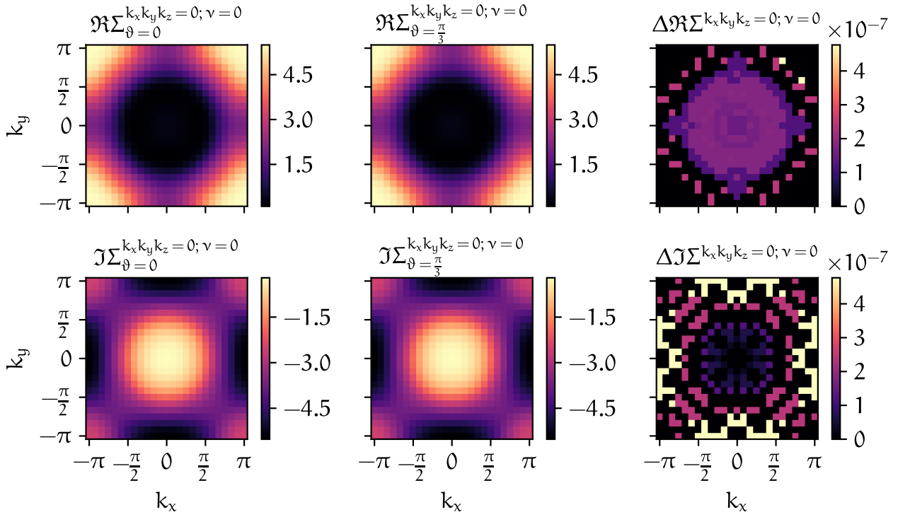
FIGURE 4.5 – Differences (third column) between the two-band calculation without a rotation ( \vartheta = 0 , first column) and a calculation, where the input data was rotated before the D \Gamma A calculation and subsequently rotated back by a factor of \vartheta = \frac{\pi}{3} (second column) for both the real and imaginary part of the self-energy (first and second row, respectively).
