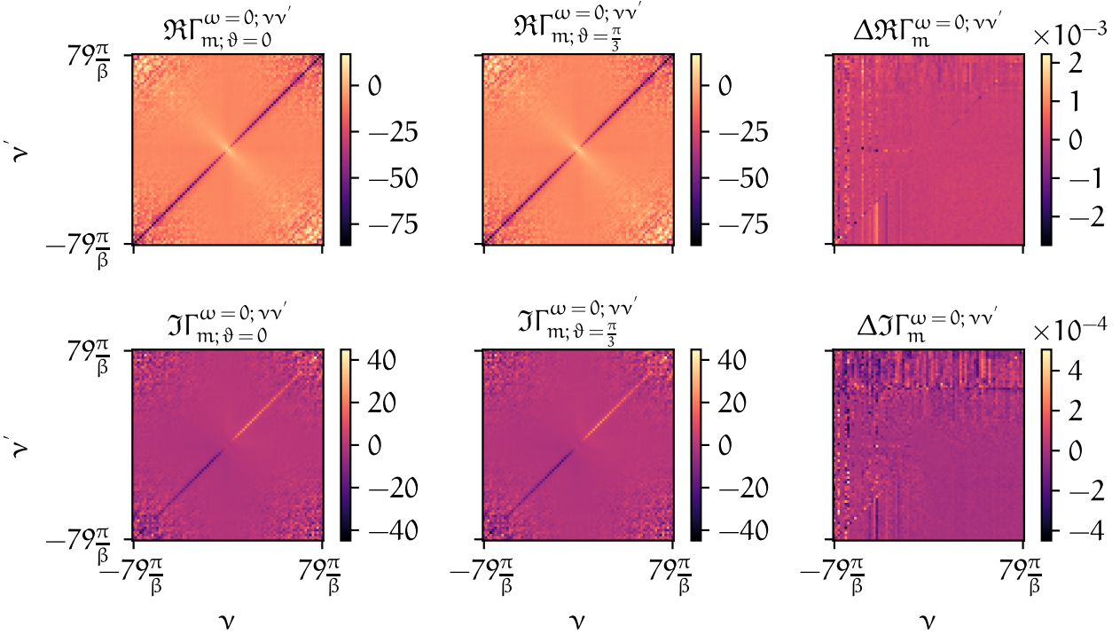
FIGURE 4.7 – Analogous to Fig. 4.6 but for the magnetic spin combination.
