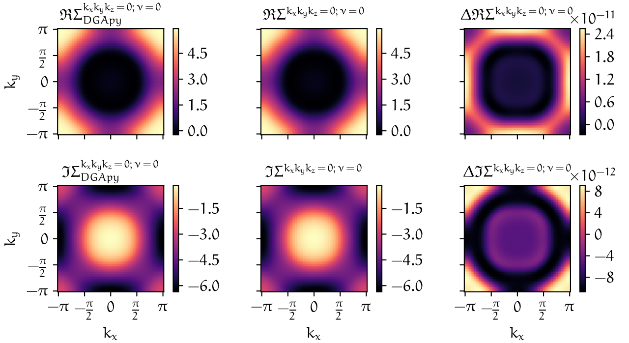
FIGURE 4.1 – Difference between the one-band self-energy of DGApy and the current implementation with the double-counting kernel of Eq. (4.2) for k_z = 0 and \nu = 0 . The result of DGApy can be seen in the very left column, the result of the current implementation in the second column. The difference between both, i.e. \Delta\Sigma = \Sigma_{\text{DGApy}} - \Sigma , can be seen in the last column. The rows indicate the real- and imaginary part of all self-energies, respectively.
