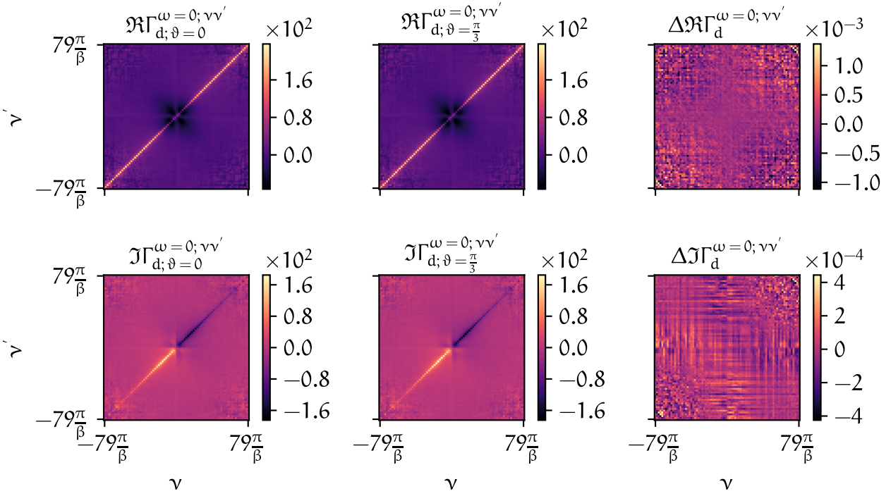
FIGURE 4.6 – Differences (third column) between the two-band calculation without a rotation ( \vartheta = 0 , first column) and a calculation, where the input data was rotated before the D \Gamma A calculation and subsequently rotated back by a factor of \vartheta = \pi/3 (second column) for both the real and imaginary part of the local irreducible vertex \Gamma_d^{\omega=0; \nu\nu'} (first and second row, respectively) in the density spin combination.
