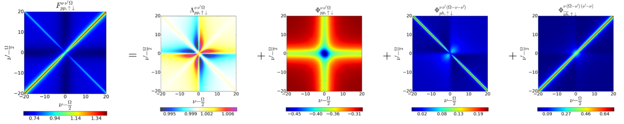
FIGURE 3.14 – Numerical SIAM results for all local vertices contained in the parquet equation Eq. (3.32) for vanishing transfer frequency \Omega = 0 , taken from Ref. [52]. In our convention, \Omega should be replaced by \omega .
