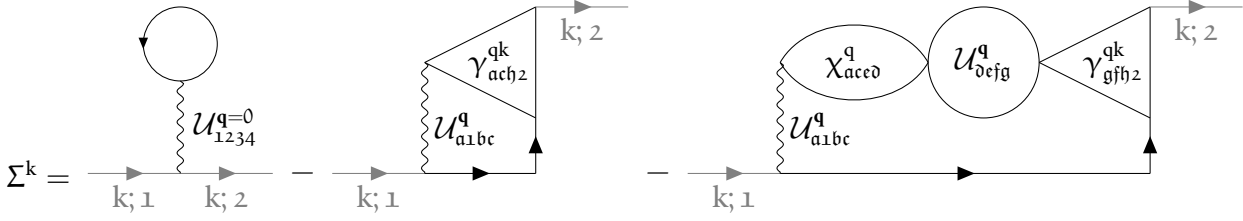
FIGURE 3.13 – Interaction-reducible form of the Schwinger-Dyson equation (3.63) with three-leg vertices.
