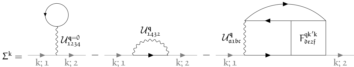
FIGURE 1.12 – Representation of the Schwinger-Dyson equation, see Eq. (1.55).
