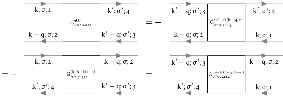
FIGURE 1.5 – Diagrammatic representation of the crossing symmetry relations in order of Eq. (1.26a) - Eq. (1.26c).
